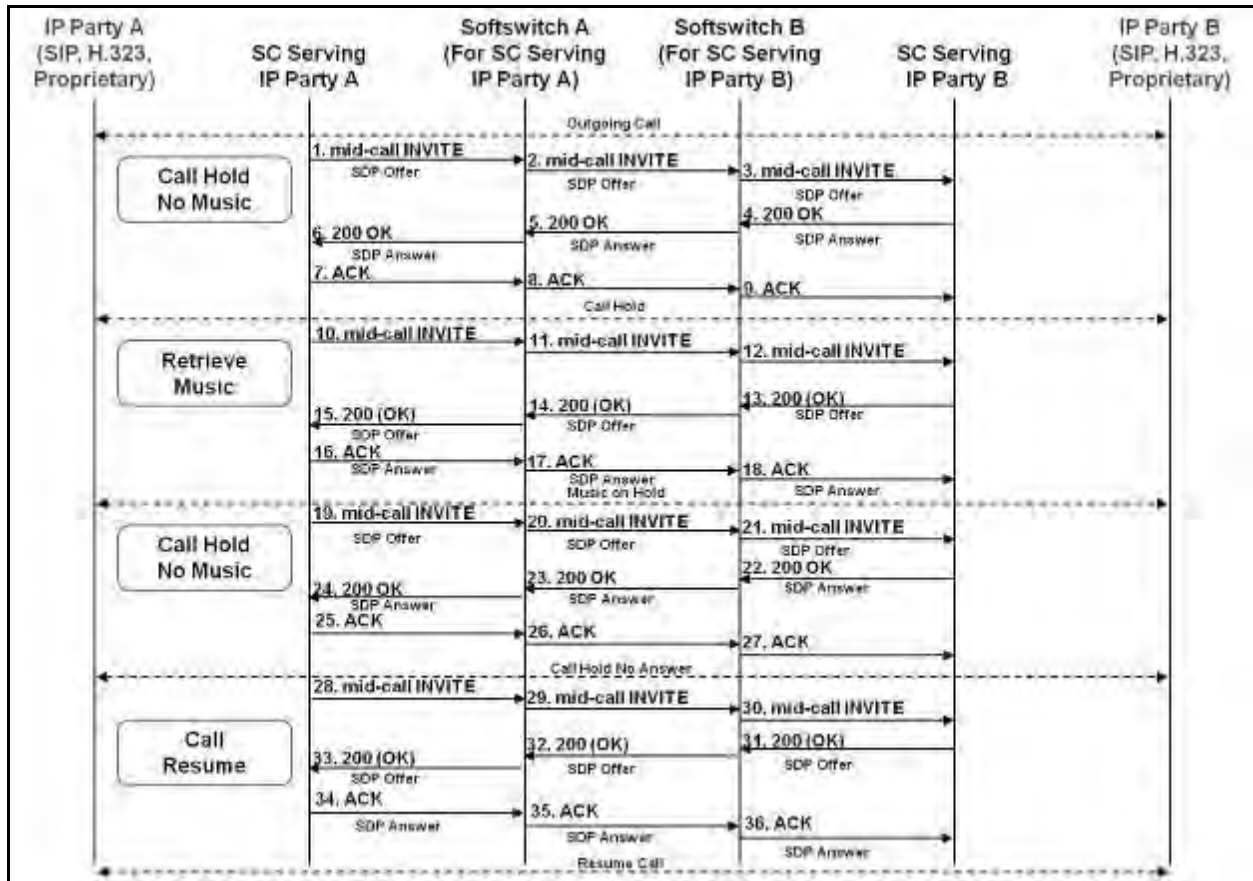
Figure 9.3-4. IP-to-IP Music on Hold (Populated INVITEs)
