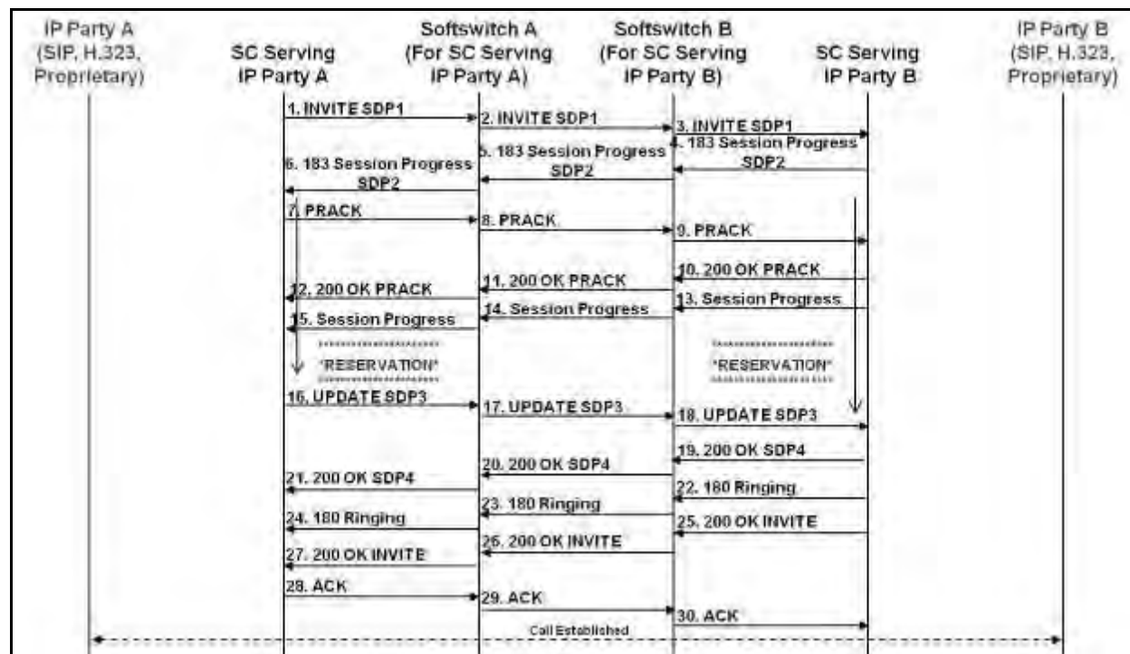
Figure 9.2-3. Successful Basic IP-to-IP Call (End-to-End Precondition)
