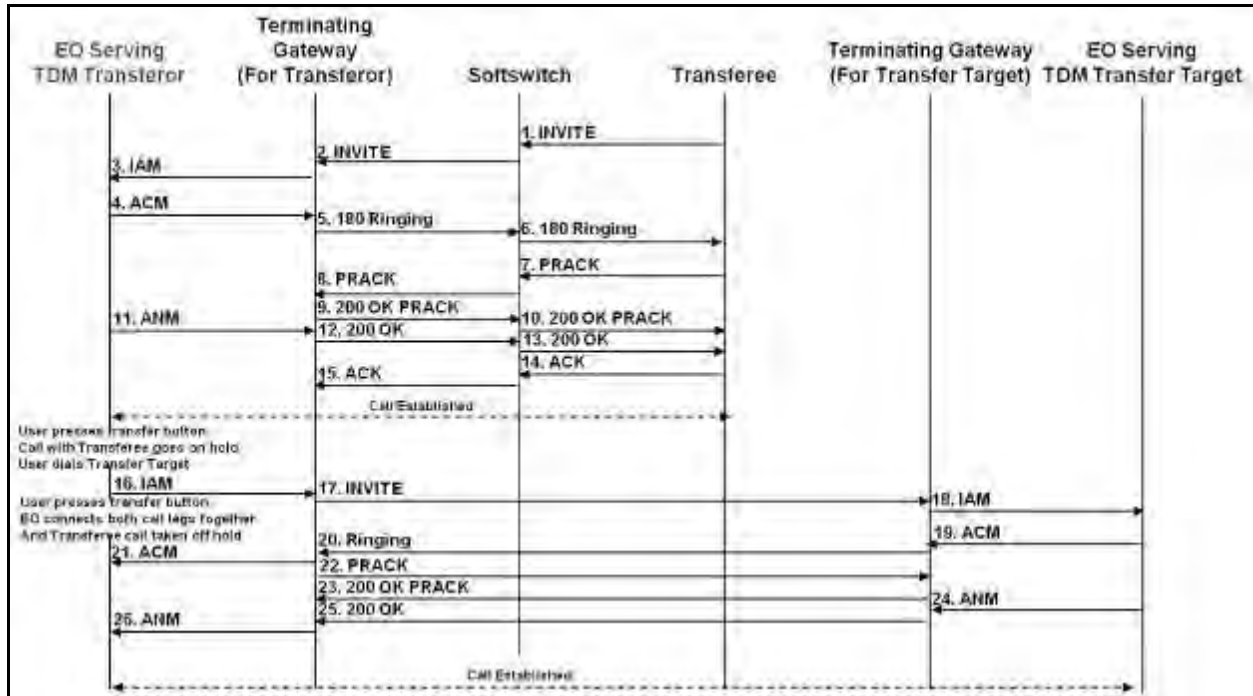
Figure 16.6-1. Unattended Call Transfer (Transferor – TDM)
