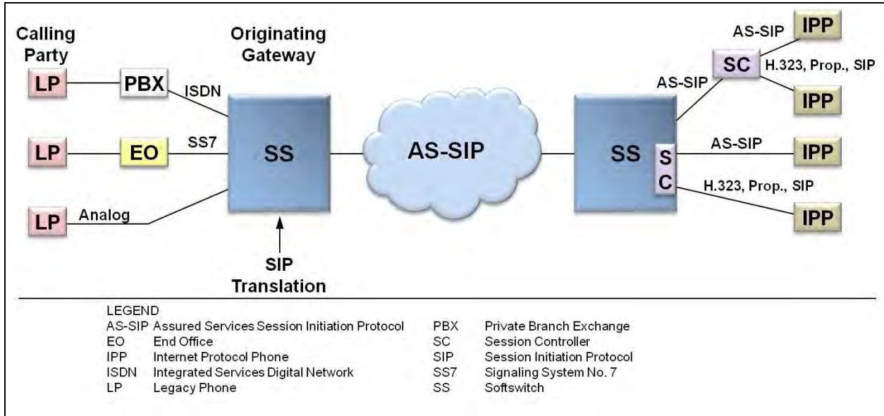
Figure 12.1-5. TDM-to-IP Call Over an IP Backbone
