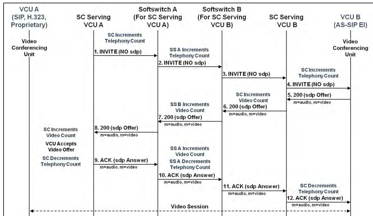
Figure 8.4-4. VCU Empty INVITE (Media Feature Tags NOT Used) – AS-SIP EI
