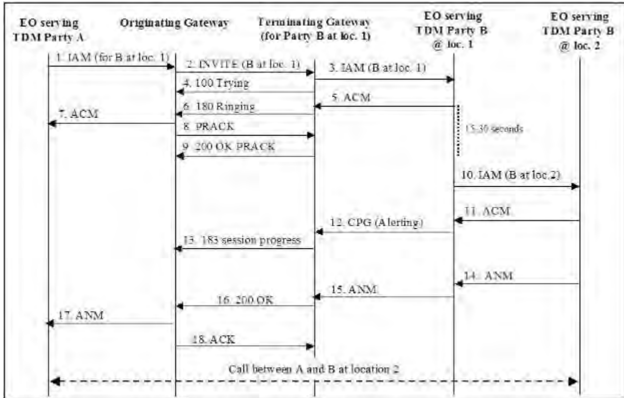
Figure 16.5-4. TDM Bridging Call Forwarding on No Answer
