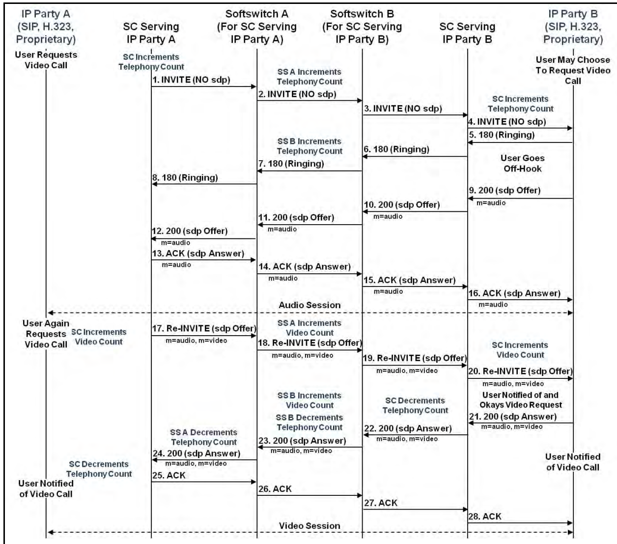
Figure 8.3-8. Empty INVITE – Caller Requests Video; Called Party Offers Audio; Caller Again Requests Video (Media Feature Tags NOT Used) – AS-SIP EI Receives Empty INVITE
