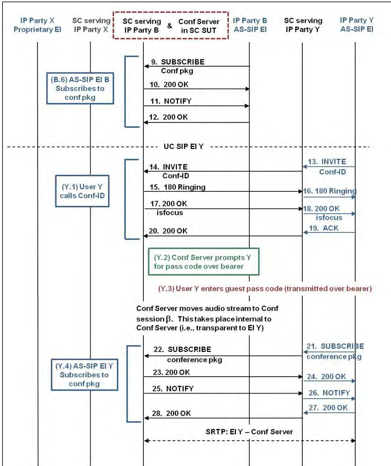
Figure 10.2-25. Scheduled Conference – Conference Server Within SC SUT, Host at AS-SIP EI (Steps 9–28)
