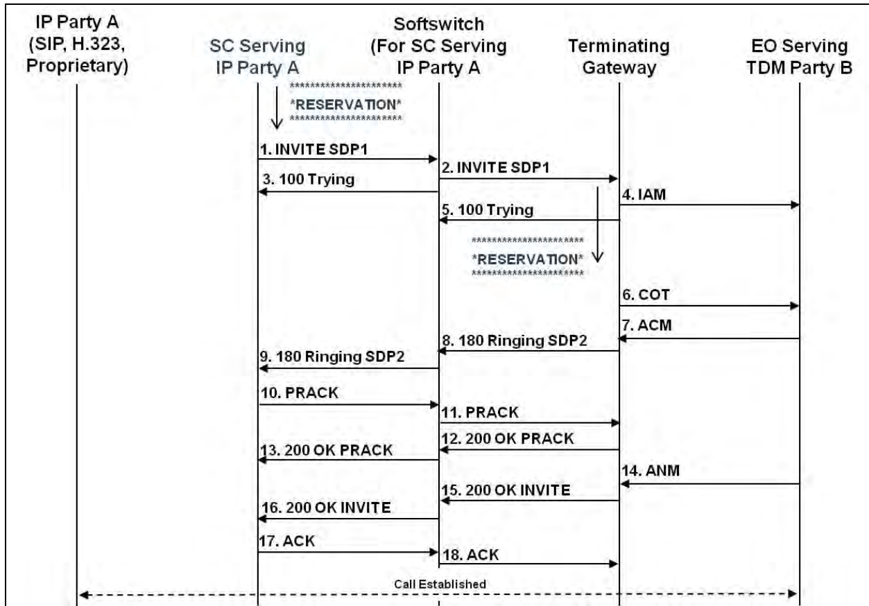
Figure 16.2-8. Successful Basic IP-to-TDM Call (Segmented Precondition)
