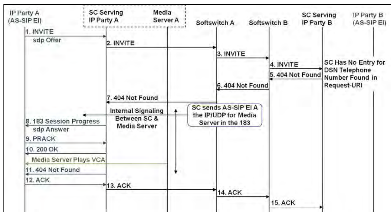
Figure 4.1-3. Originating SC Implements Playing of VCA at AS-SIP EI Upon Receipt of 404 Response From Destination SC
