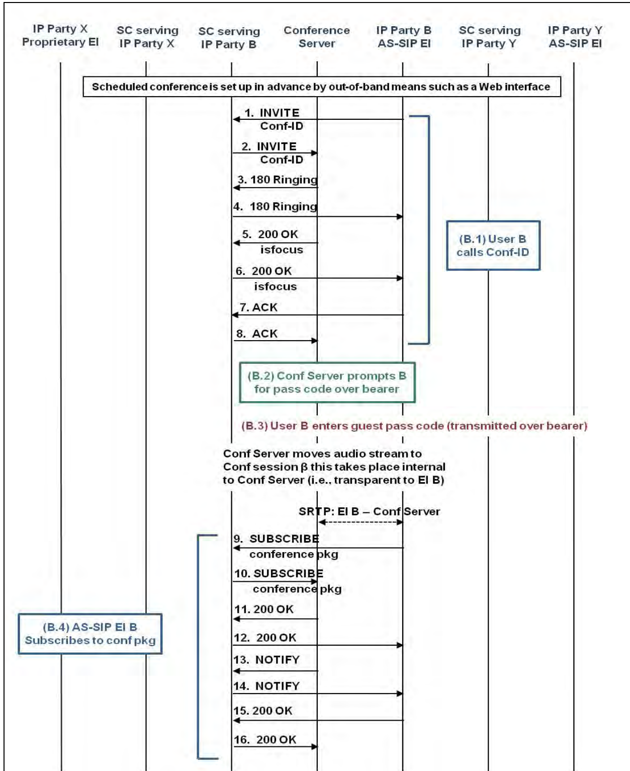
Figure 10.3-5. Scheduled Videoconference – AS-SIP Conference Server (Steps 1–16)
