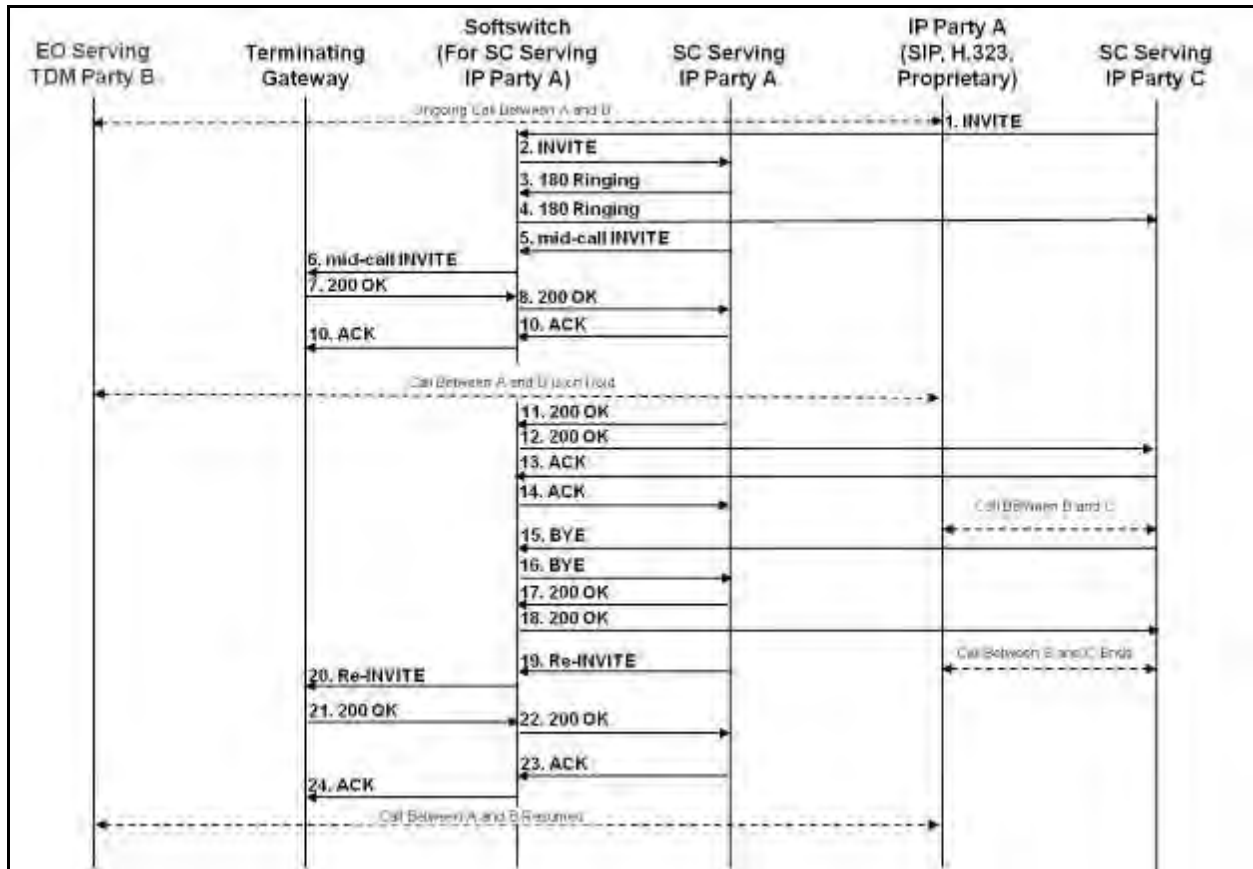
Figure 16.4-7. IP-to-TDM Call Waiting (Performed at IP Party A)
