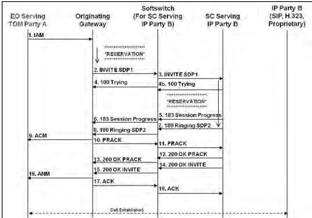
Figure 16.2-5. Successful Basic TDM-to-IP Call (Segmented Precondition)
