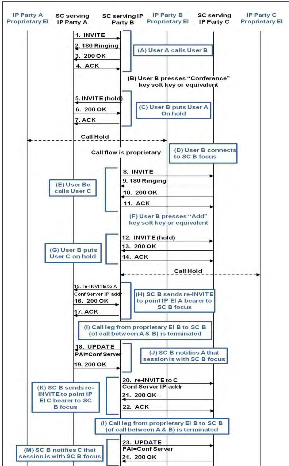
Figure 9.7-6. Three-Way Call at SC (RE-INVITE Method)
