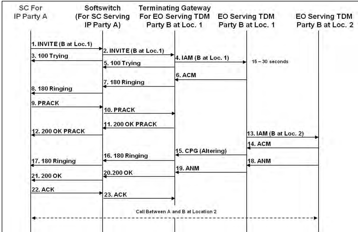
Figure 16.5-6. IP-to-TDM Call Forwarding (No Answer)
