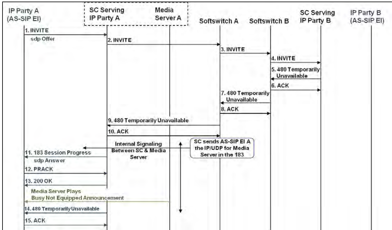
Figure 6.4-1. SC Implementation of BNEA for AS-SIP EI on Receipt of 480 Response
