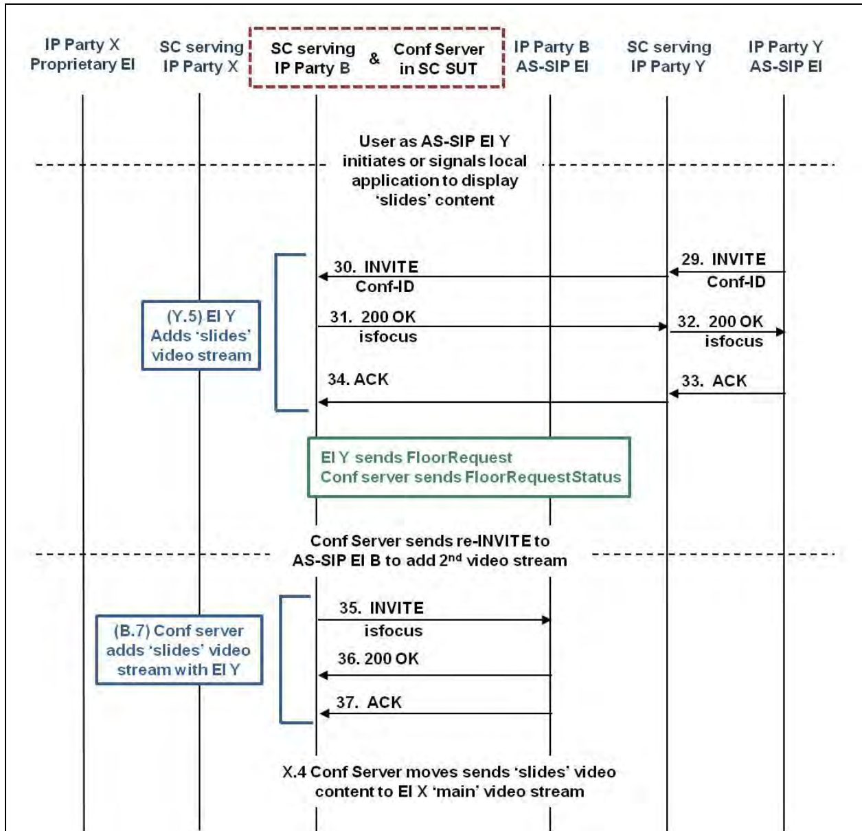
Figure 10.3-4. Scheduled Videoconference – Conference Server Within SC SUT (Steps 29–37)
