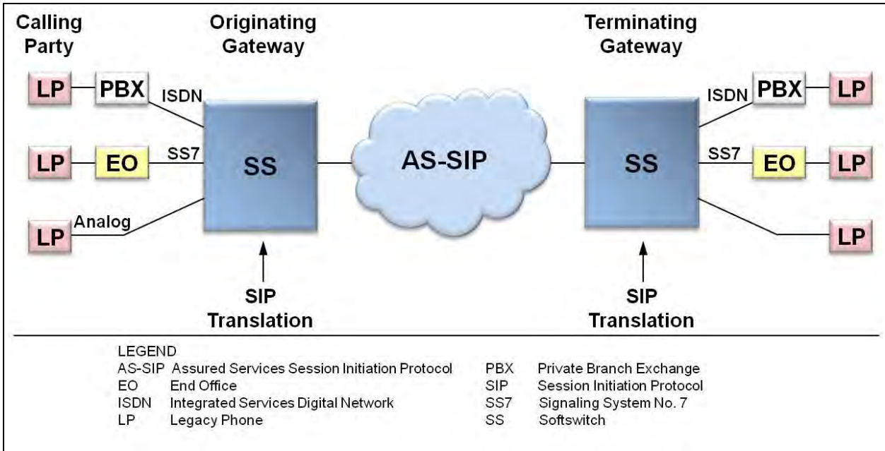
Figure 12.1-1. TDM-to-TDM Bridging Over an IP Backbone
