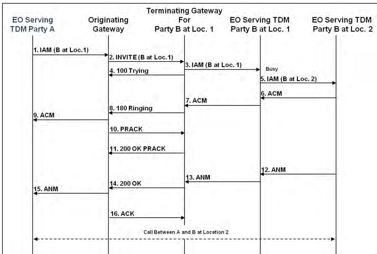
Figure 16.5-7. TDM Bridging Call Forwarding on Busy (Call Forward Signaling Occurs Within ISUP Network)
