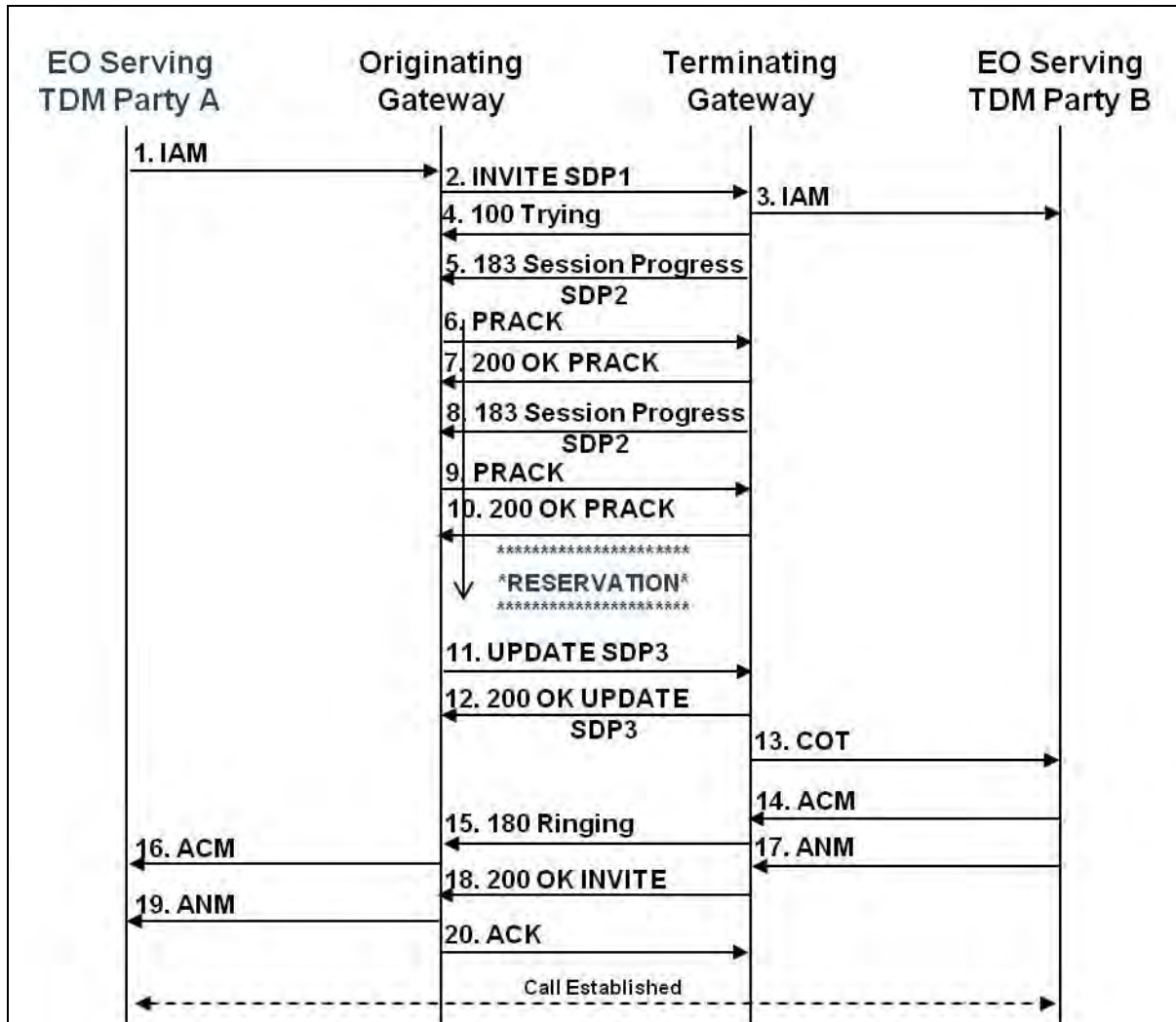
Figure 16.2-3. Successful Basic TDM Bridging Call (End-to-End Precondition)
