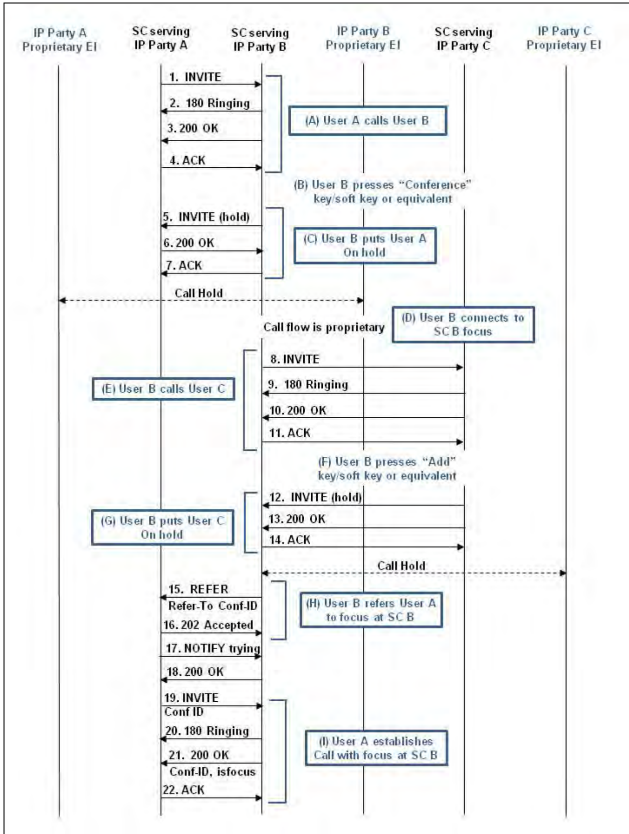
Figure 9.7-4. Three-Way Call at SC (REFER Method) (Steps 1–22)
