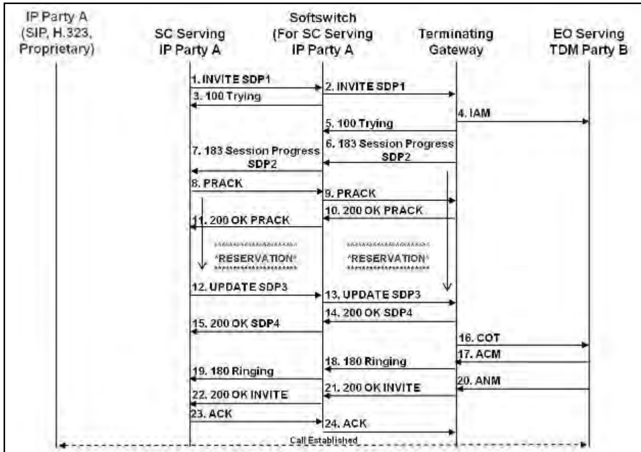
Figure 16.2-9. Successful Basic IP-to-TDM Call (End-to-End Precondition)
