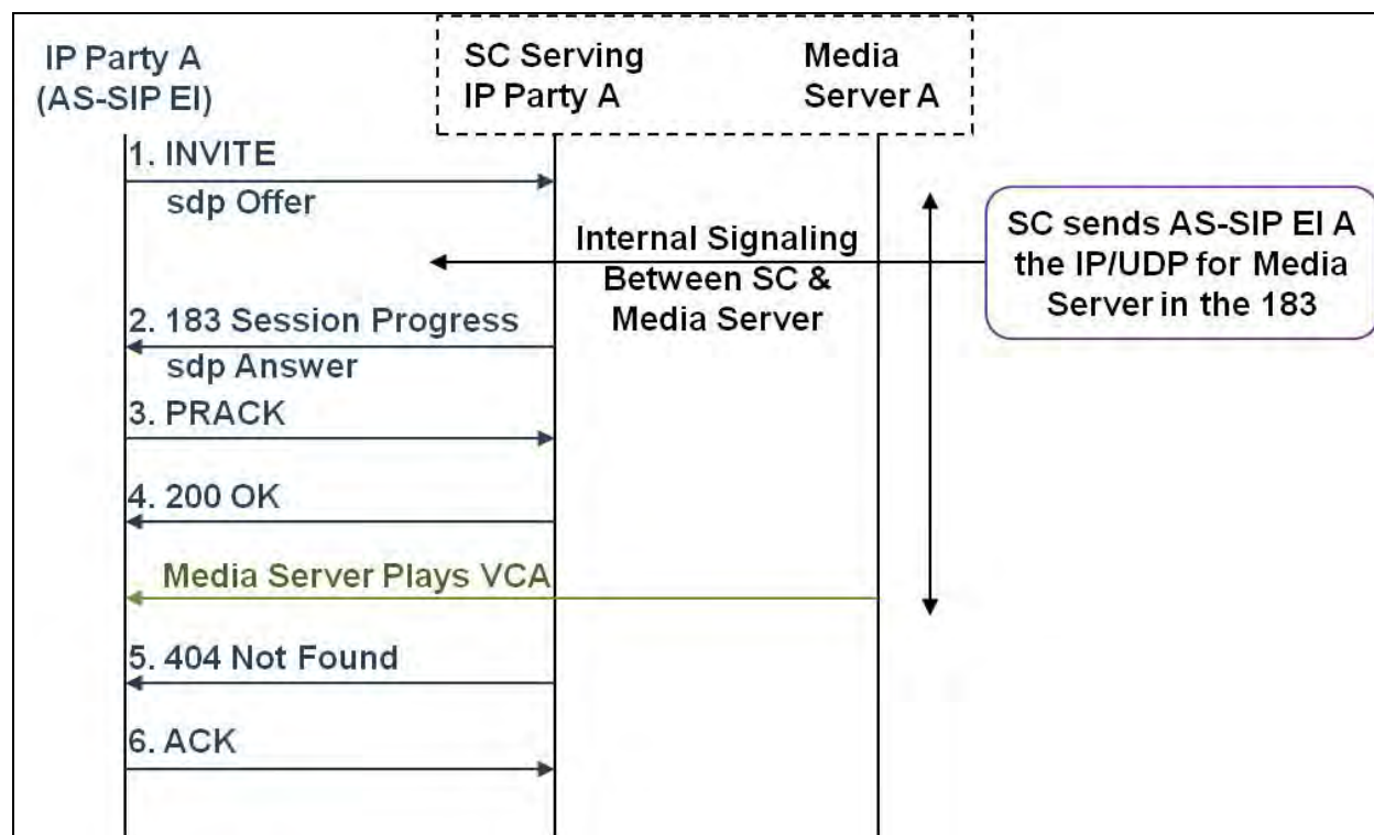
Figure 4.6-1. Originating SC Implements Playing of VCA at AS-SIP EI When SC Is Unable To Create a Full 10-Digit DSN Number for the Userinfo Part of the Request-URI Field
