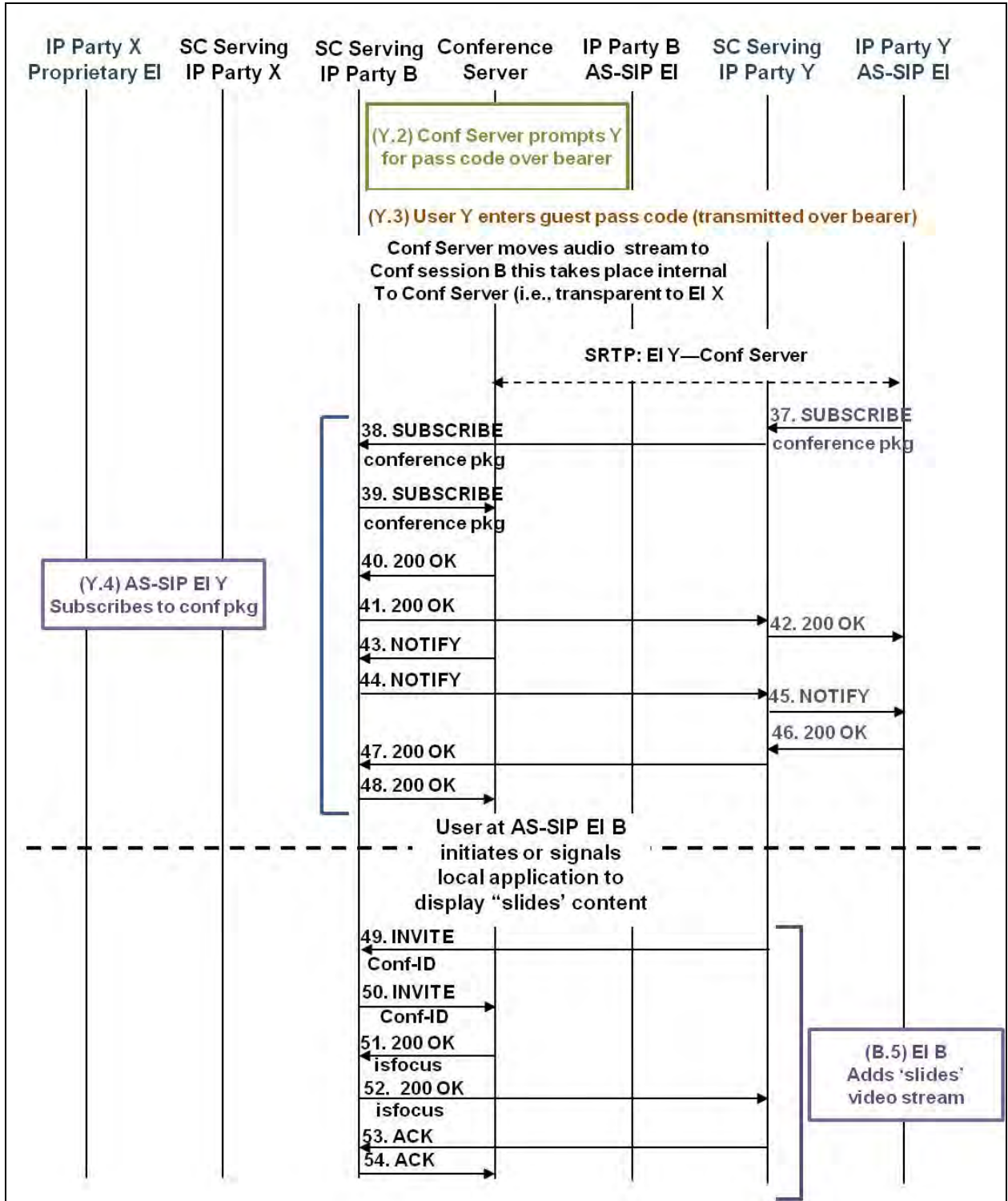
Figure 10.3-7. Scheduled Videoconference – AS-SIP Conference Server (Steps 37–54)
