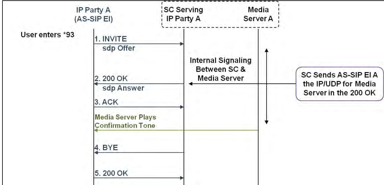
Figure 9.5-7. Call Flow Between AS-SIP EI and SC Using Star Code To Deactivate Call Forward on No Answer
