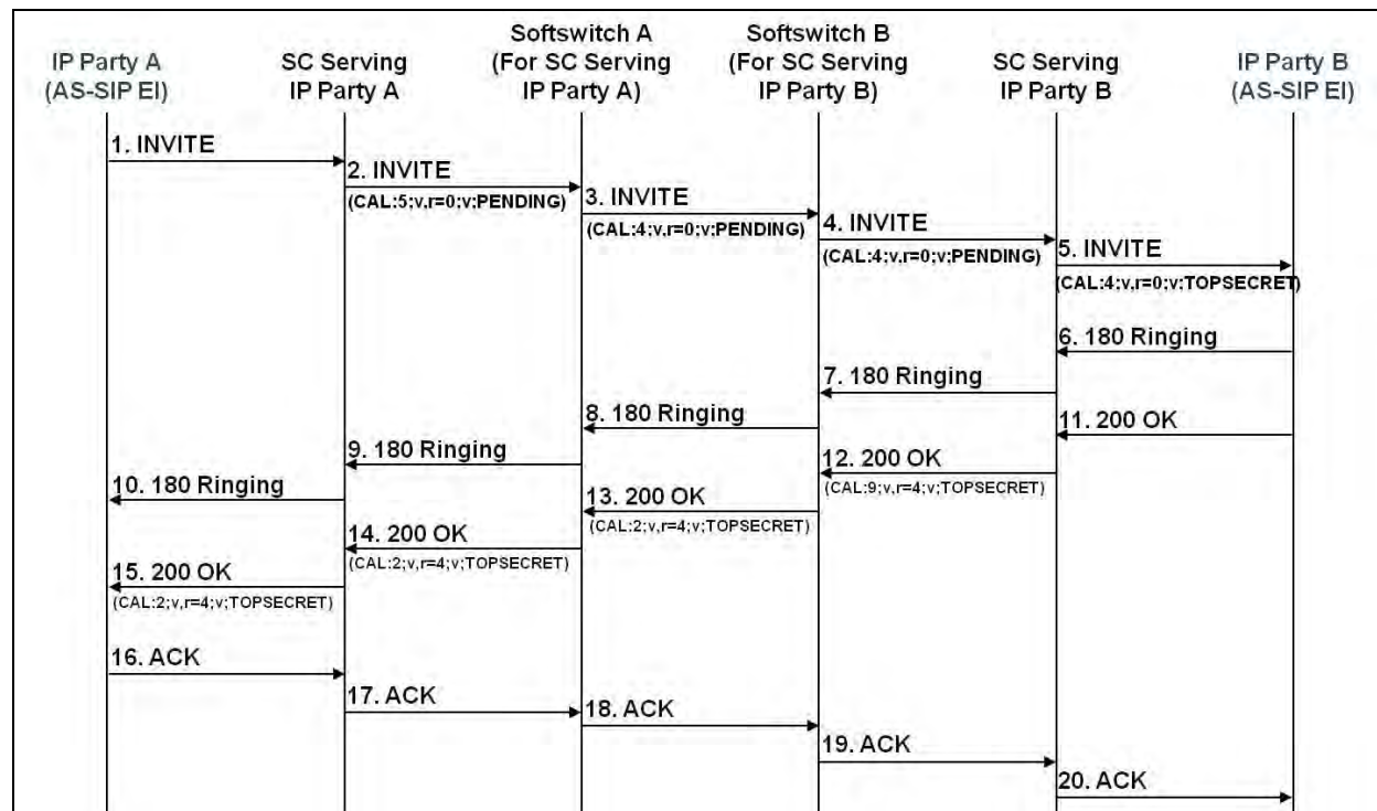
Figure 4.9-1. Example of CAL Session Establishment Using Variable Mode
