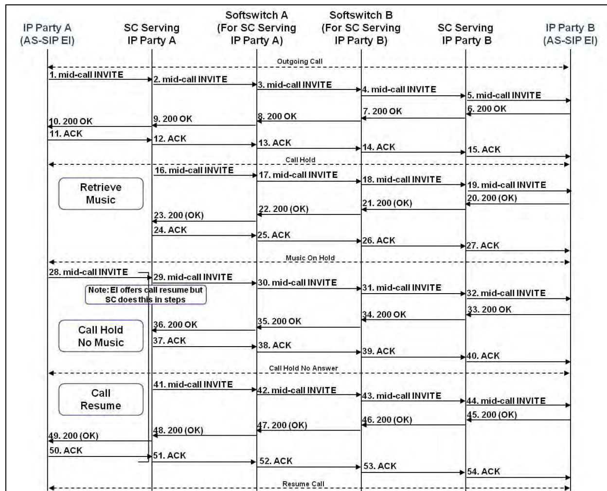
Figure 9.3-6. IP-to-IP Music on Hold (AS-SIP EIs)
