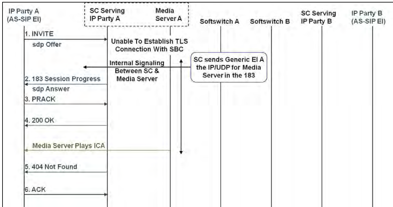
Figure 4.1-1. SC Implements Playing of ICA at AS-SIP EI
