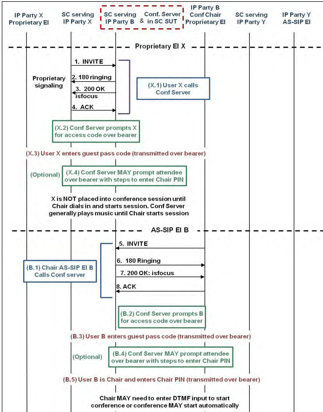
Figure 10.2-15. Reservationless Conference – Conference Server Within SC SUT, Conference Chair at AS-SIP EI (Steps 1–8)
