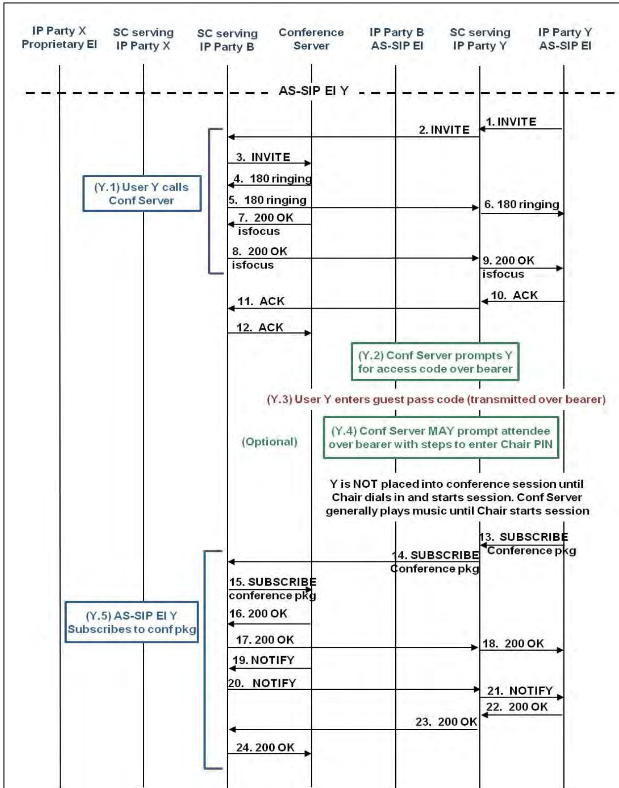
Figure 10.2-19. Reservationless Conference – AS-SIP Conference Server, Conference Chair at Proprietary EI (Steps 1–24)
