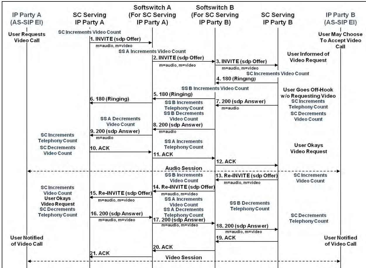
Figure 8.3-3. INVITE With sdp Video Offer – Called Party Accepts Video After 200 Response
