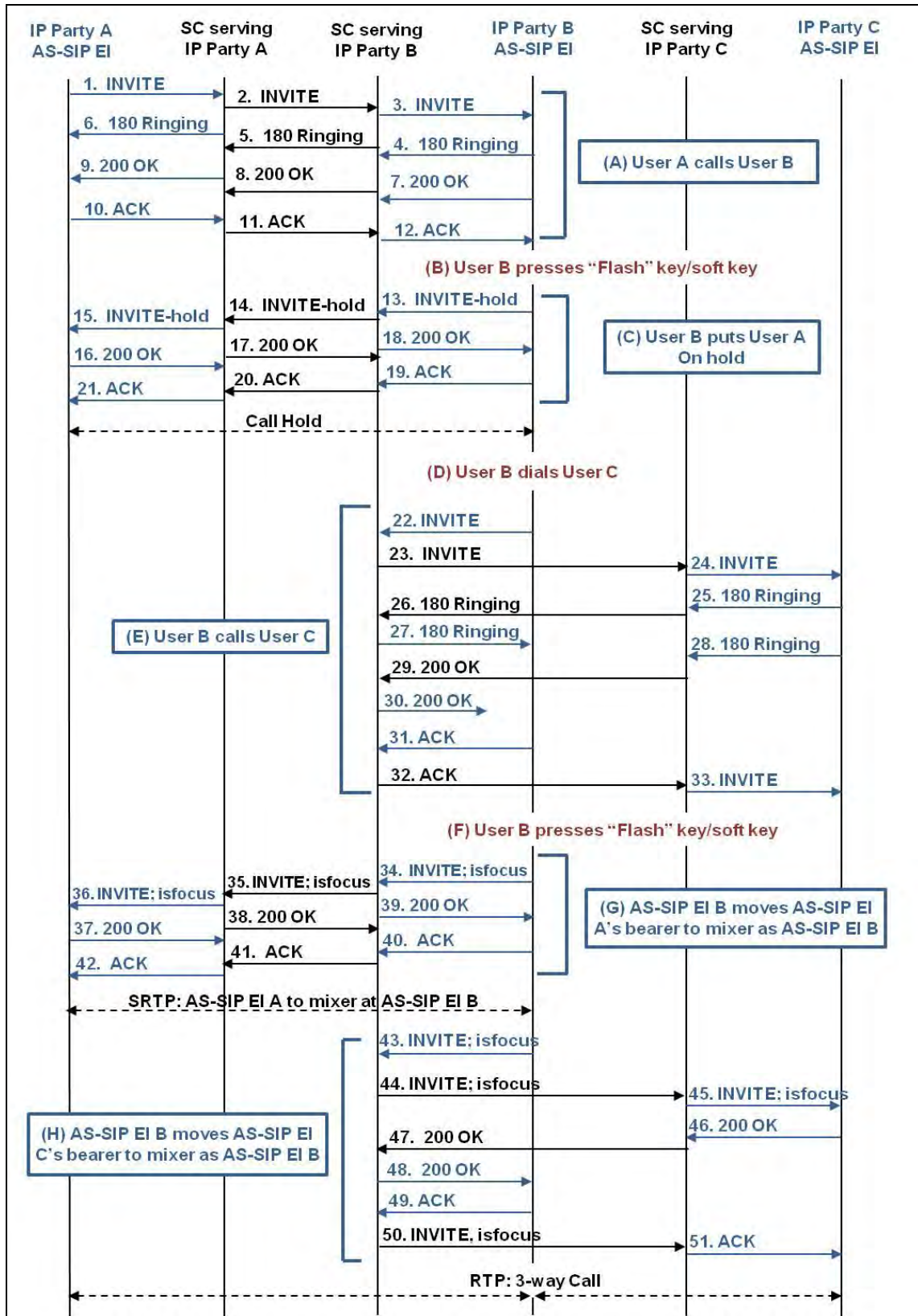
Figure 9.7-3. AS-SIP EI Provides Focus for Three-Way Call
