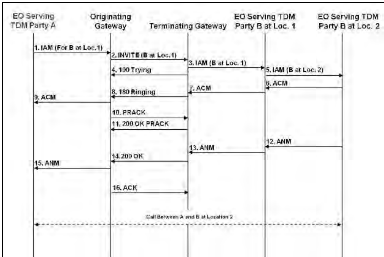
Figure 16.5-1. TDM Bridging Call Forward Unconditional (Call Forward Signaling Occurs Within ISUP Network)
