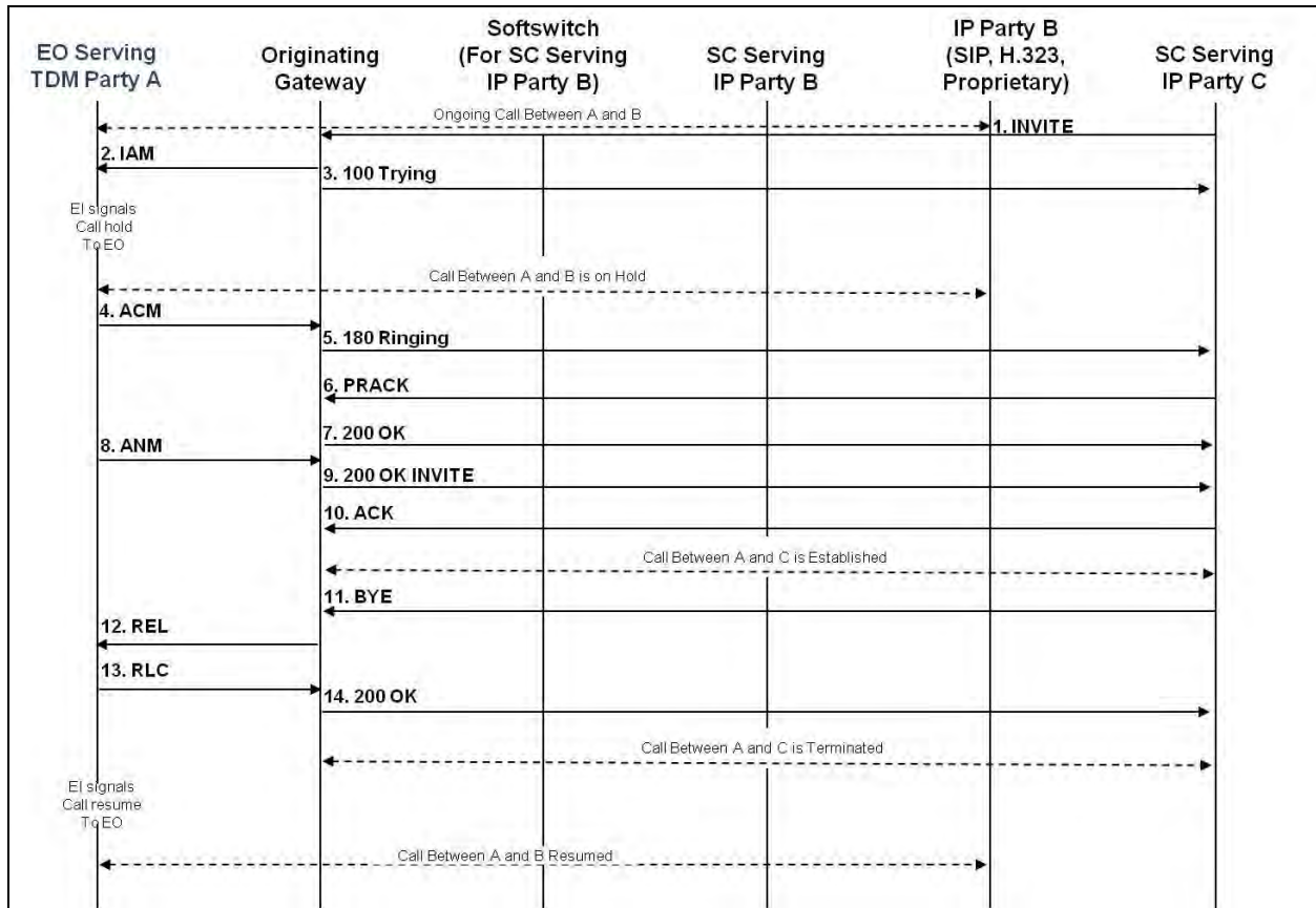
Figure 16.4-5. TDM-to-IP Call Waiting (Performed at TDM Party A)
