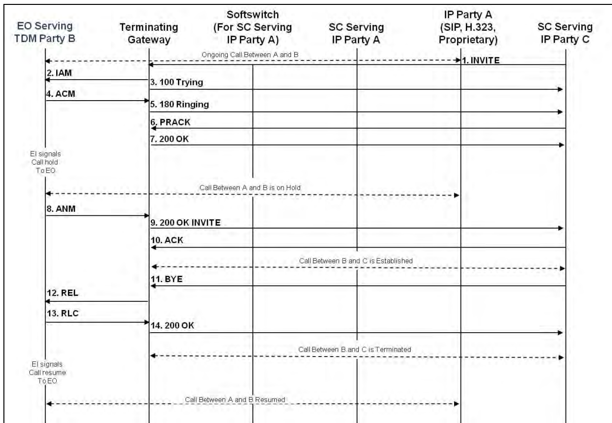
Figure 16.4-6. IP-to-TDM Call Waiting (Performed at TDM Party B)
