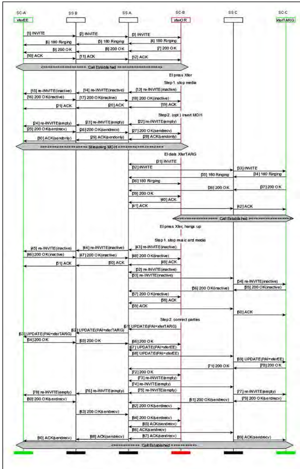
Figure 9.6-4. Attended Call Transfer for IP EI (INVITE and re-INVITE Method)
