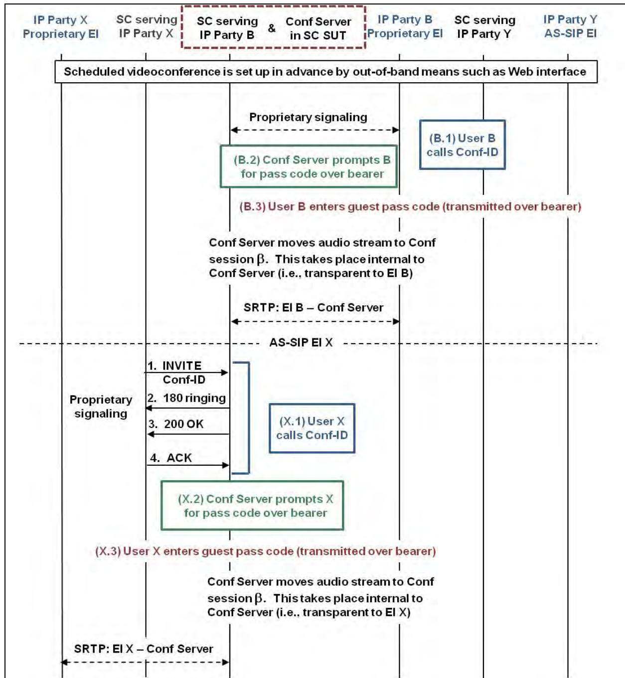
Figure 10.2-22. Scheduled Conference – Conference Server Within SC SUT, Host at Proprietary EI (Steps 1–4)
