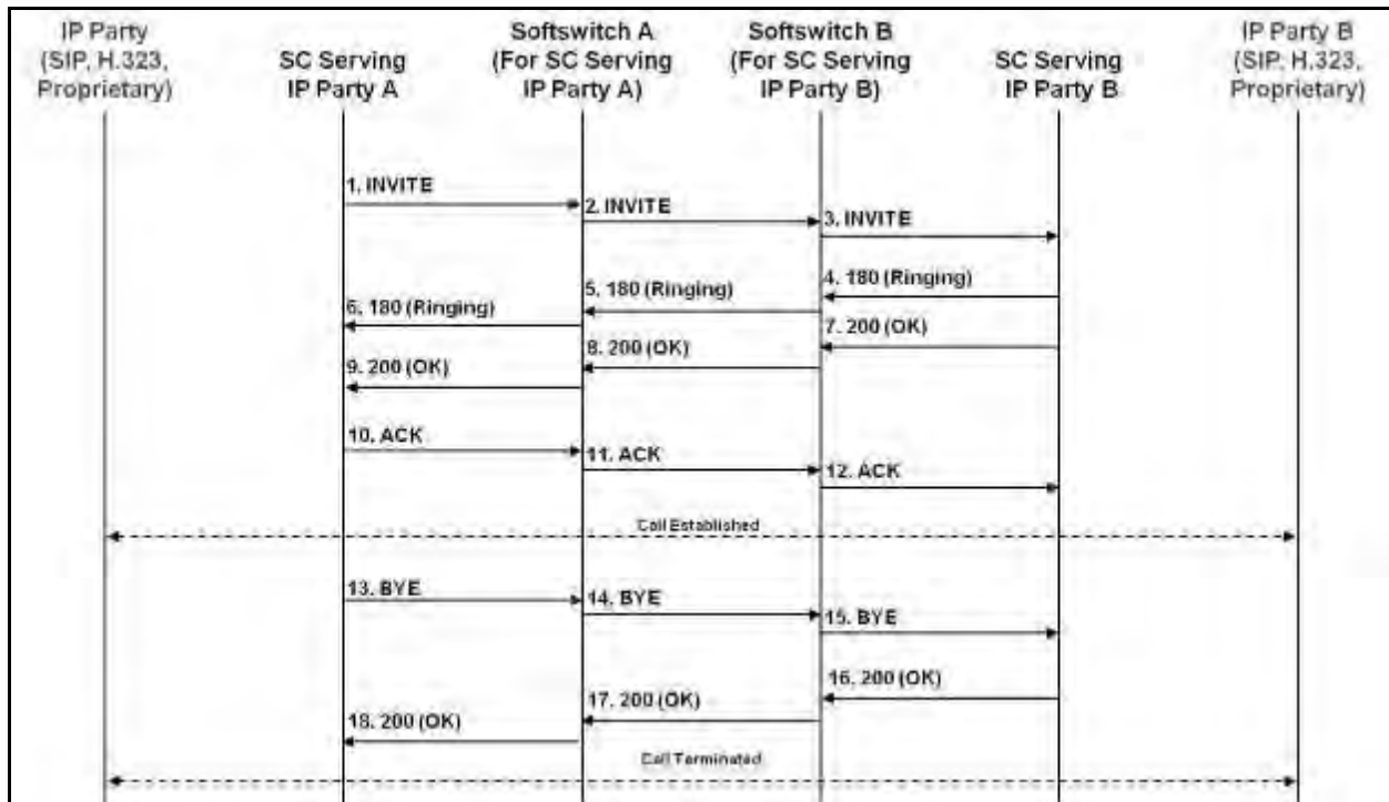
Figure 9.2-1. Successful Basic IP-to-IP Call (No Reliable Provisional Responses, No Preconditions)
