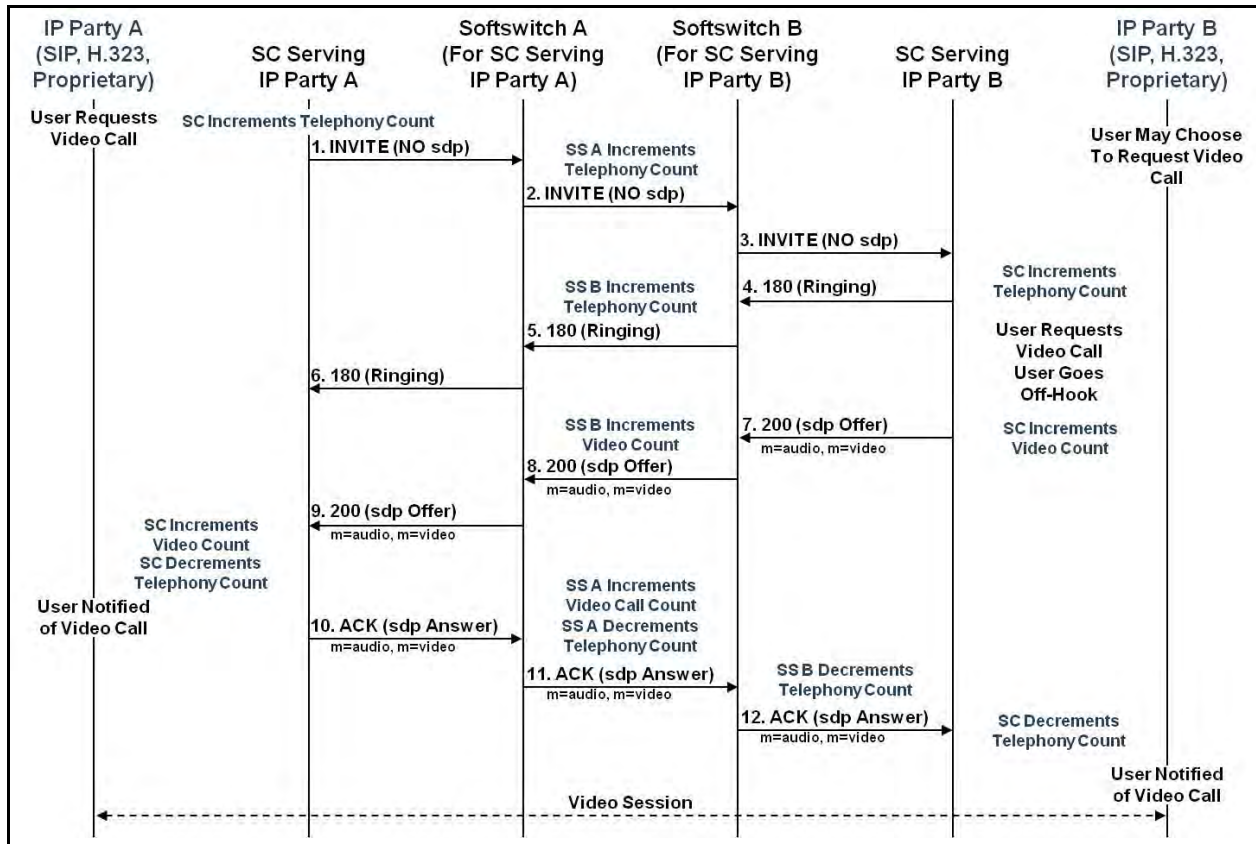
Figure 8.3-5. Empty INVITE – Caller Requests Video; Called Party Offers Video (Media Feature Tags NOT Used)
