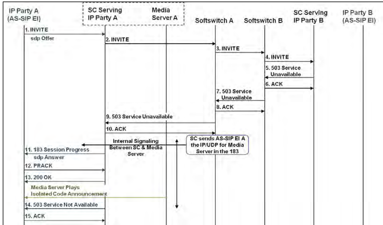
Figure 6.1-3. SC Implementation of ICA for AS-SIP EI on Receipt of 503 Response
