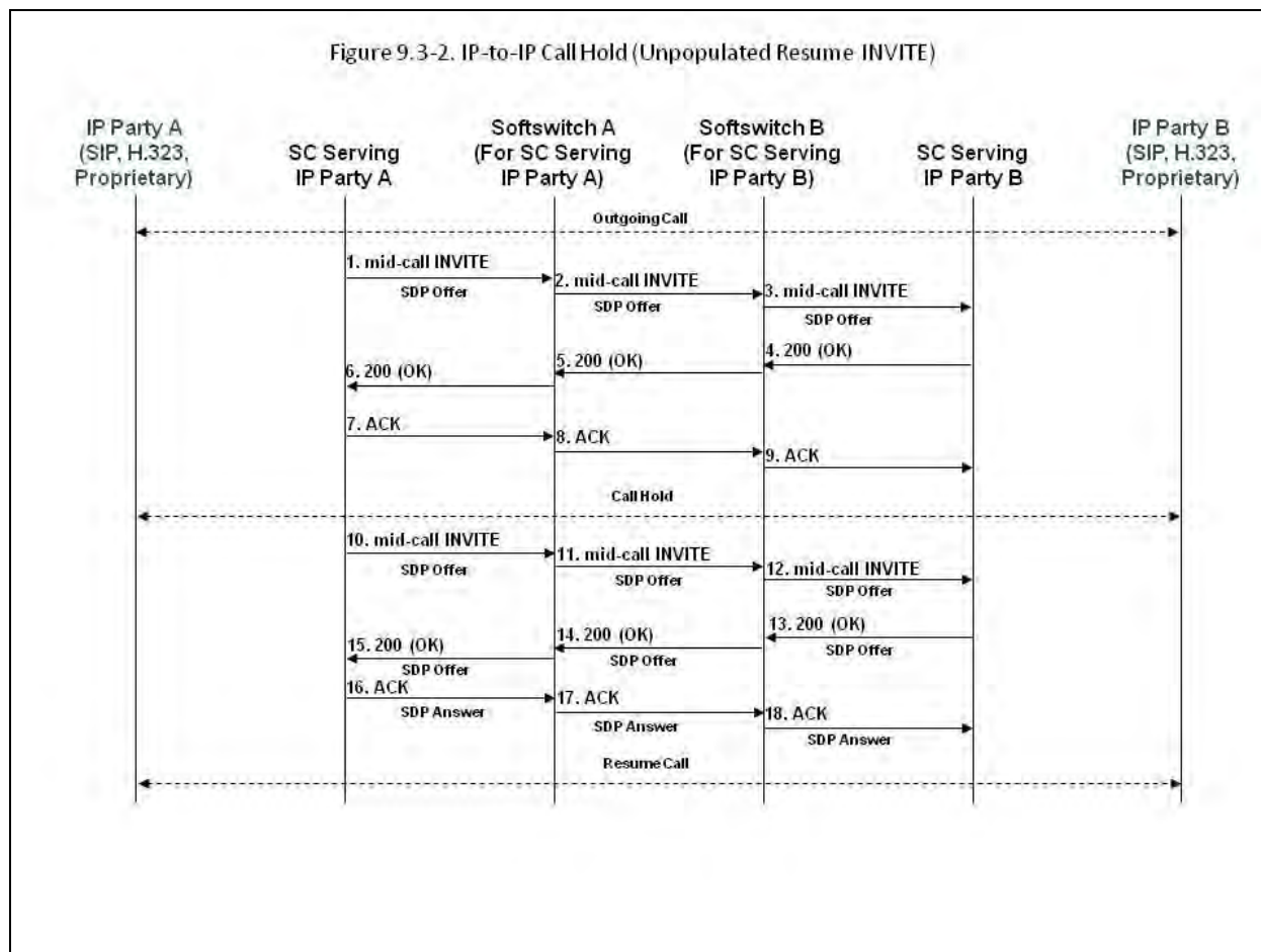
Figure 9.3-2. IP-to-IP Call Hold (Unpopulated Resume INVITE)
