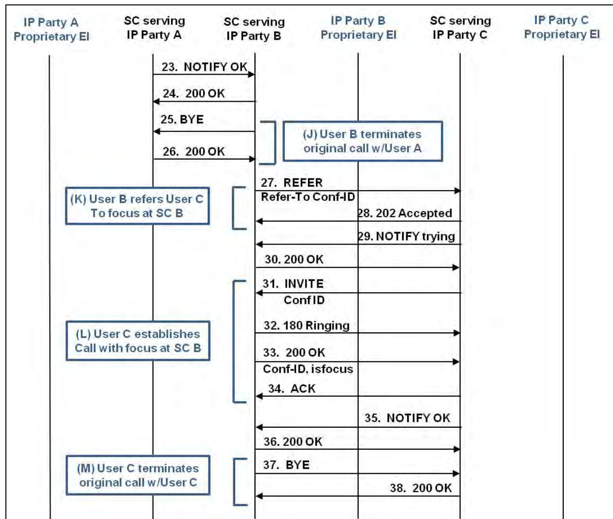
Figure 9.7-5. Three-Way Call at SC (REFER Method) (Steps 23–38)
