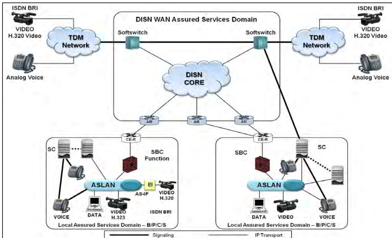
Figure 2-1. Network-Level AS-SIP Signaling Design
