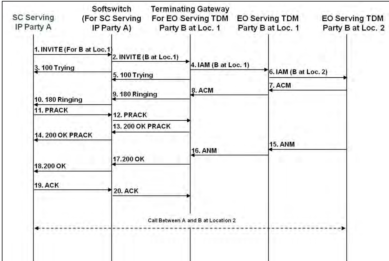
Figure 16.5-3. IP-to-TDM Call Forwarding (Call Forward Signaling Occurs in ISUP Network)
