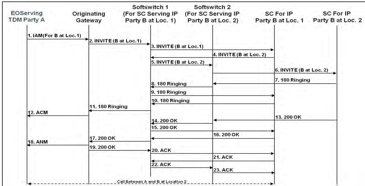
Figure 16.5-2. TDM-to-IP Call Forwarding
