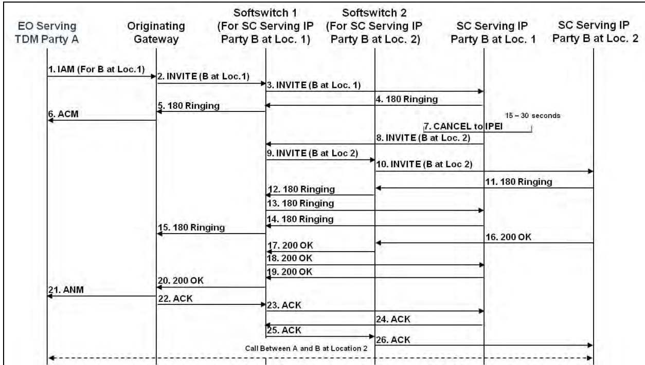
Figure 16.5-5. TDM-to-IP Call Forwarding on No Answer
