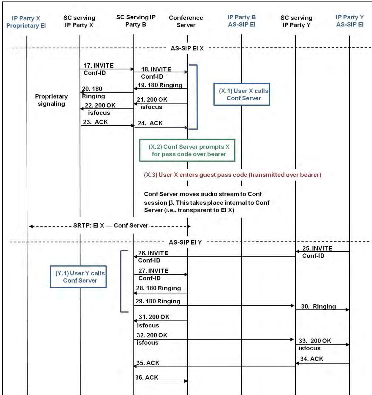
Figure 10.2-29. Scheduled Conference – AS-SIP Conference Server, Host at AS-SIP EI (Steps 17–36)
