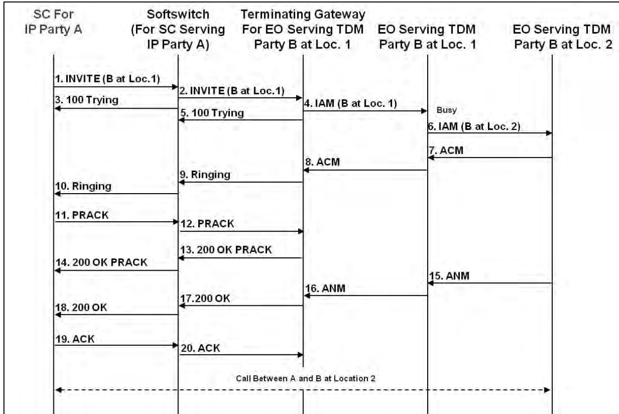
Figure 16.5-8. TDM-to-IP Call Forwarding on Busy
