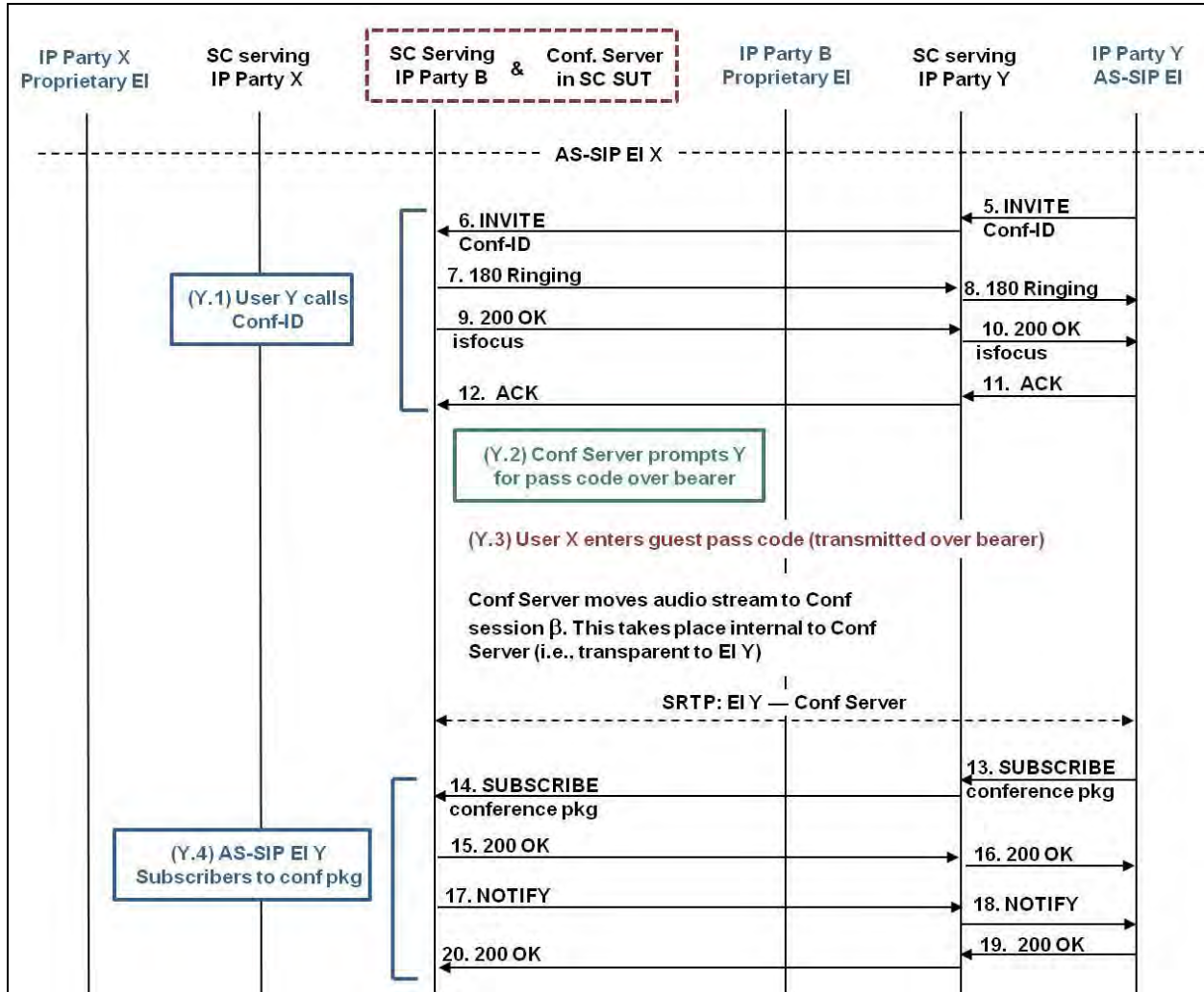
Figure 10.2-23. Scheduled Conference – Conference Server Within SC SUT, Host at Proprietary EI (Steps 5–20)
