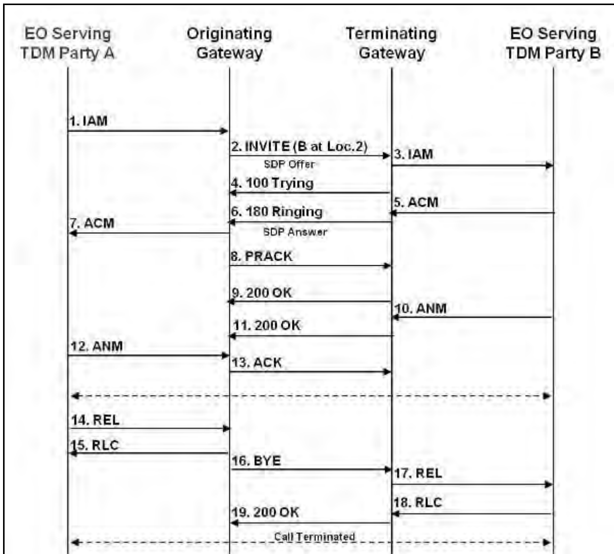
Figure 16.2-1. Successful Basic TDM Bridging Call (No Preconditions)
