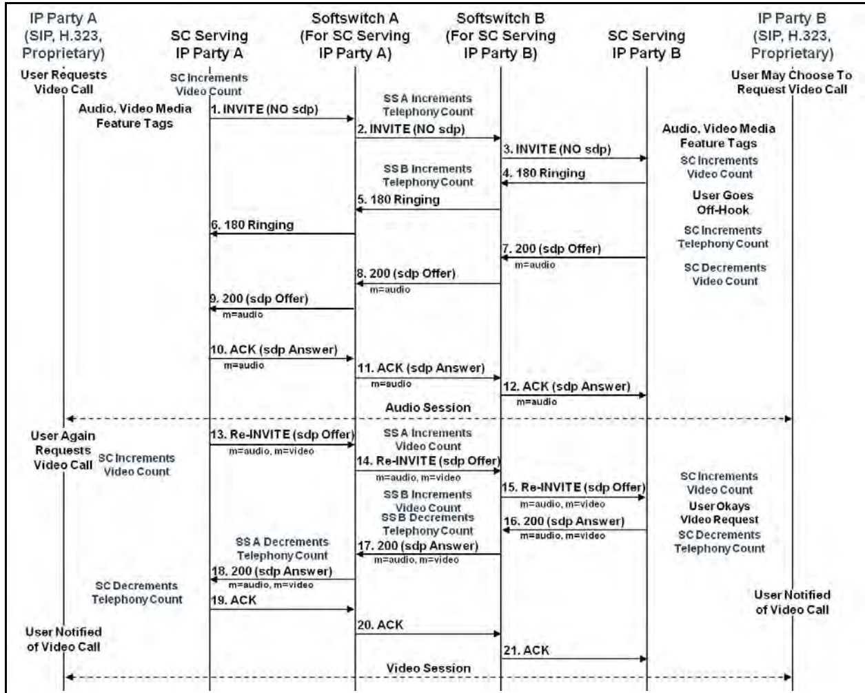
Figure 8.3-11. Empty INVITE – Caller Requests Video; Called Party Offers Audio – Calling Party Again Requests Video (Media Feature Tags Used by Originating SC and Terminating SC)
