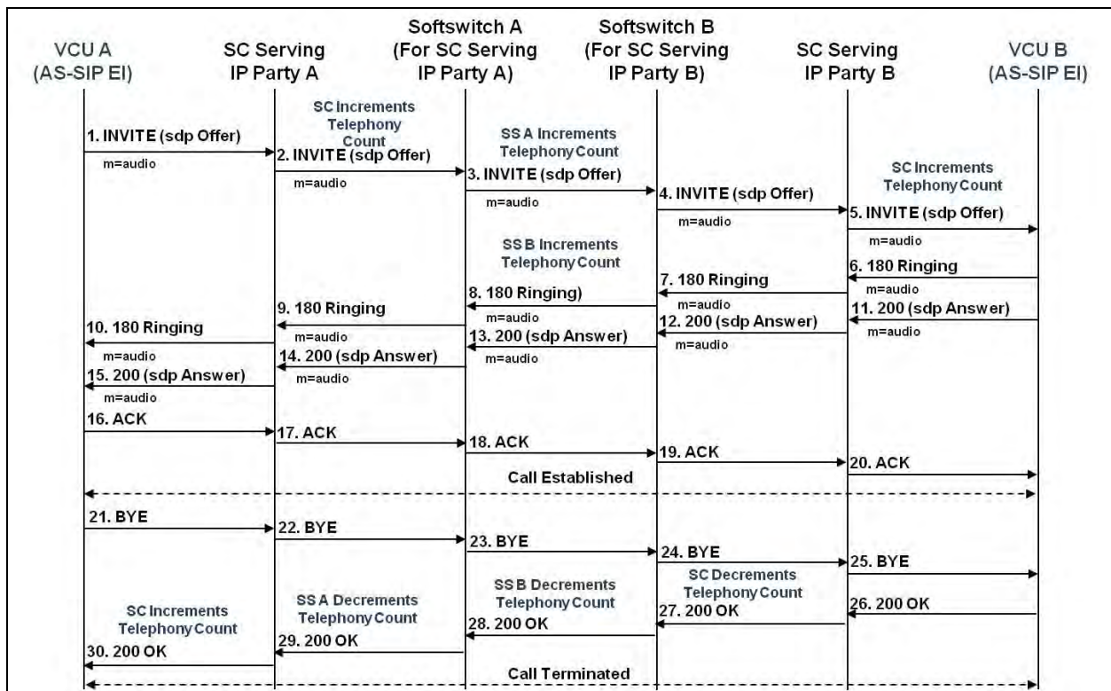
Figure 9.2-2. Successful Basic IP-to-IP Call (No Reliable Provisional Responses, No Preconditions) (AS-SIP EIs)
