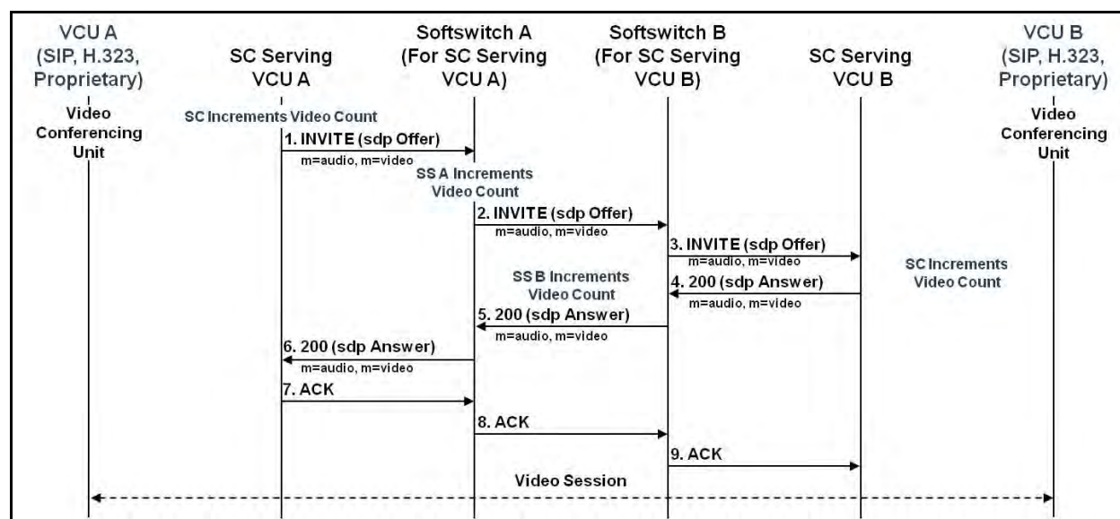
Figure 8.4-1. VCU INVITE With sdp Video Offer
