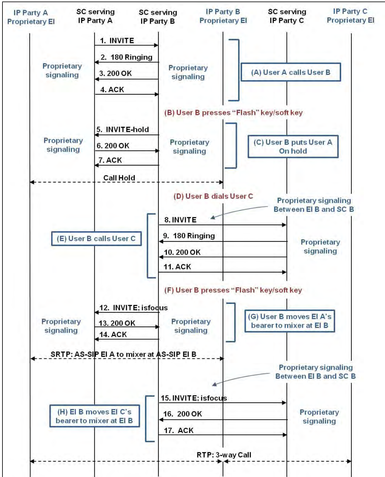
Figure 9.7-2. Proprietary EI Provides Focus for Three-Way Call
