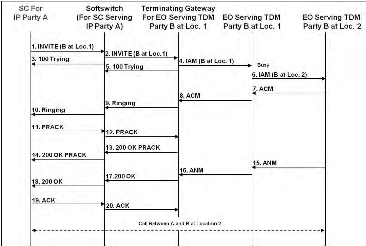
Figure 16.5-9. IP-to-TDM Call Forwarding on Busy
