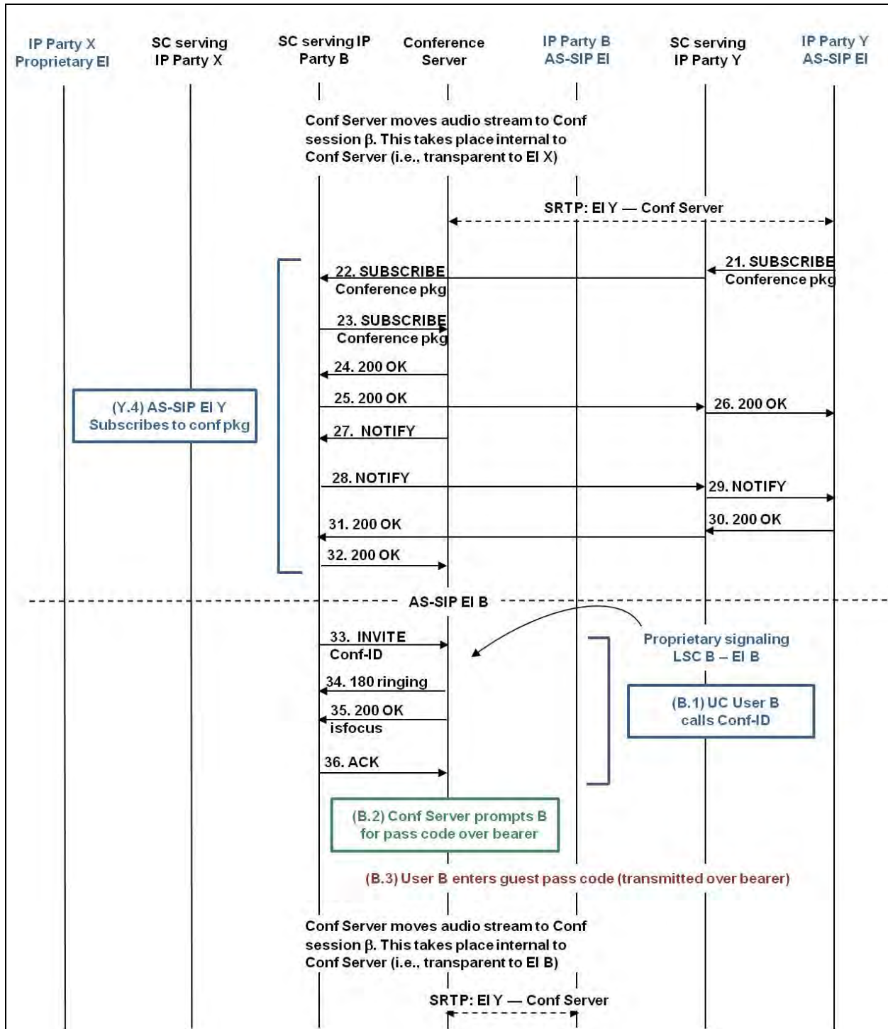
Figure 10.2-27. Scheduled Conference – AS-SIP Conference Server, Host at Proprietary EI (Steps 21–36)
