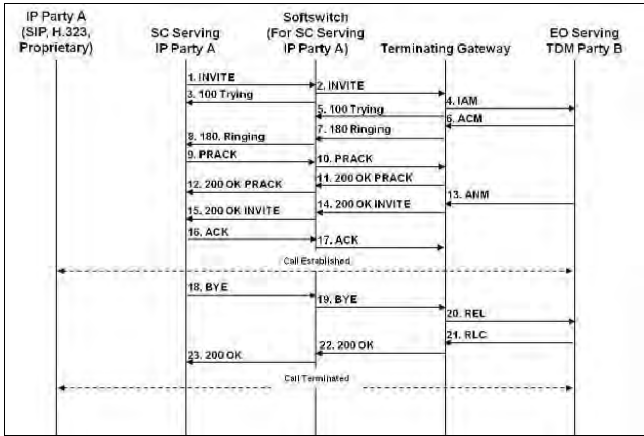
Figure 16.2-7. Successful Basic IP-to-TDM Call (No Preconditions)
