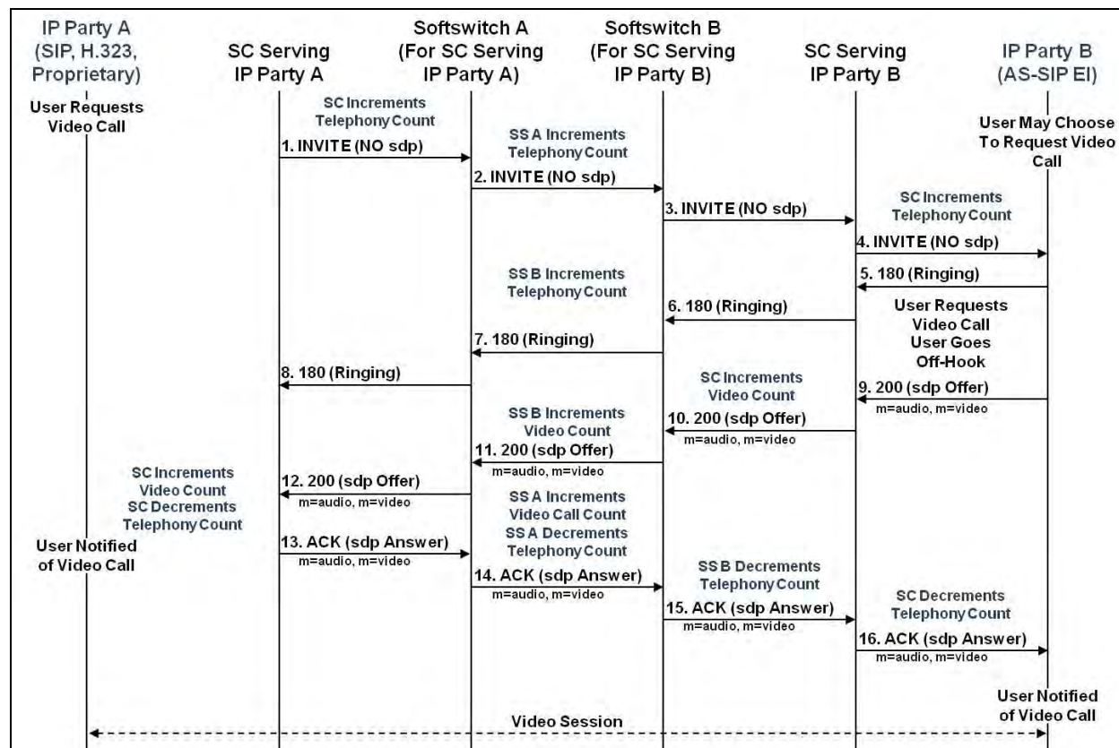
Figure 8.3-6. Empty INVITE – Caller Requests Video; Called Party Offers Video (Media Feature Tags NOT Used) – AS-SIP EI Receives Empty INVITE
