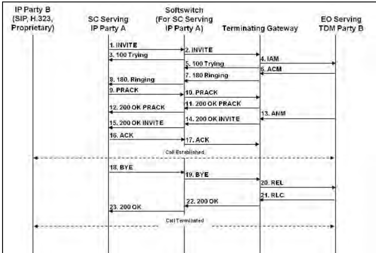
Figure 16.2-4. Successful Basic TDM-to-IP Call (No Preconditions)
