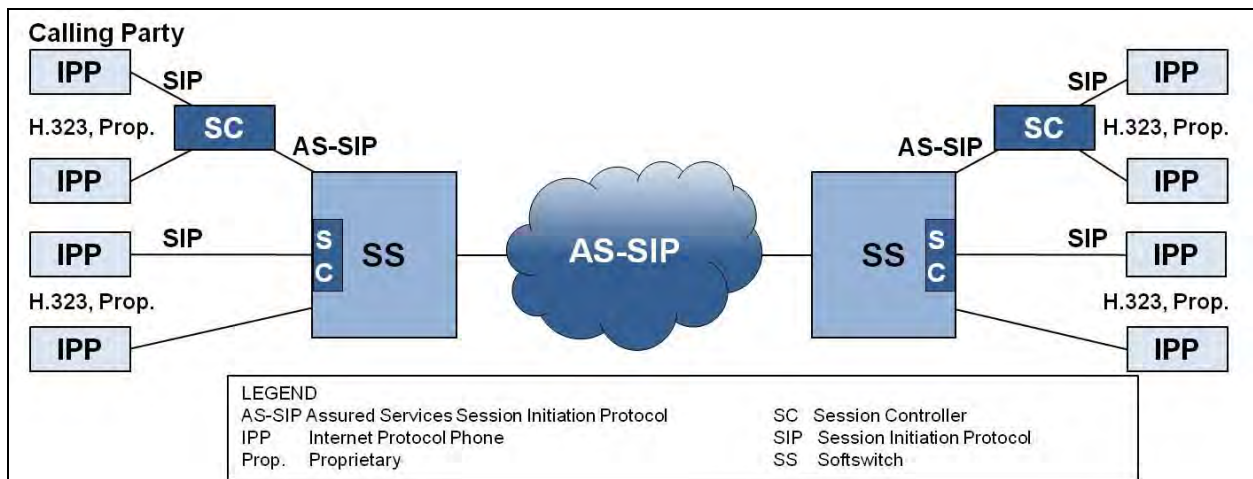
Figure 3-1. IP-to-IP Calls Over an IP Backbone
