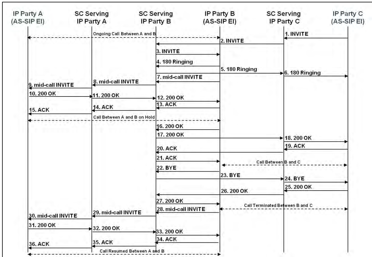
Figure 9.4-2. IP-to-IP Call Waiting (AS-SIP EI)
