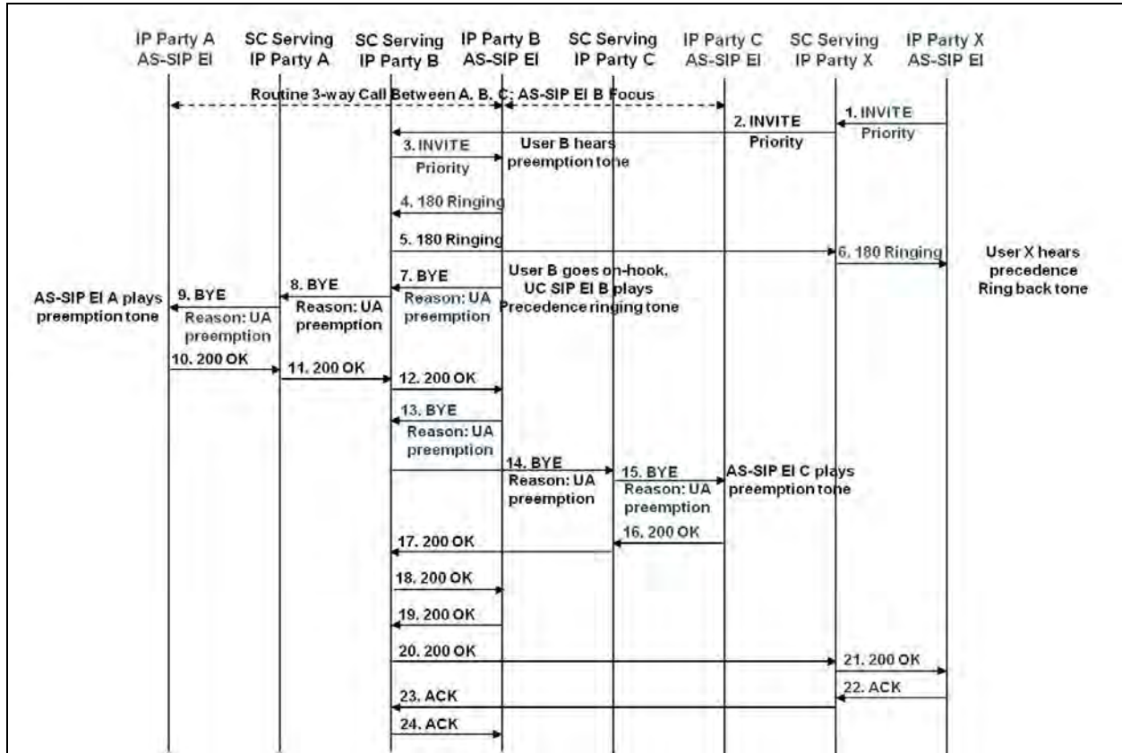
Figure 9.7-1. Endpoint Preemption of Three-Way Call
