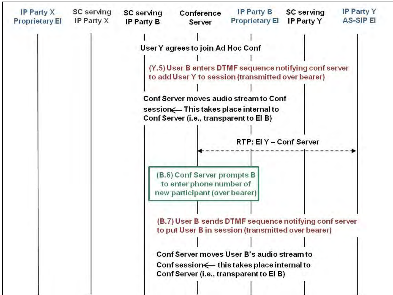
Figure 10.2-9. Ad Hoc Conference – AS-SIP Conference Server, Conference Initiator at Proprietary EI
