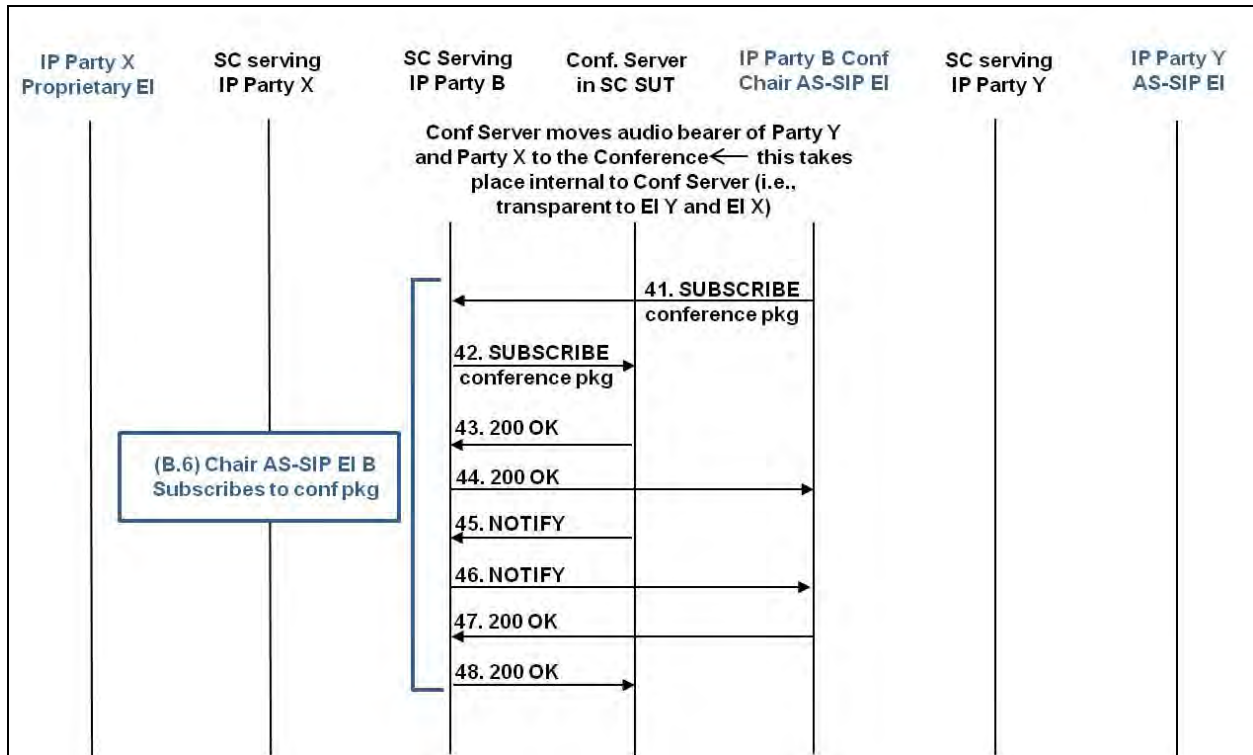
Figure 10.2-21. Reservationless Conference – AS-SIP Conference Server, Conference Chair at Proprietary EI (Steps 41–48)
