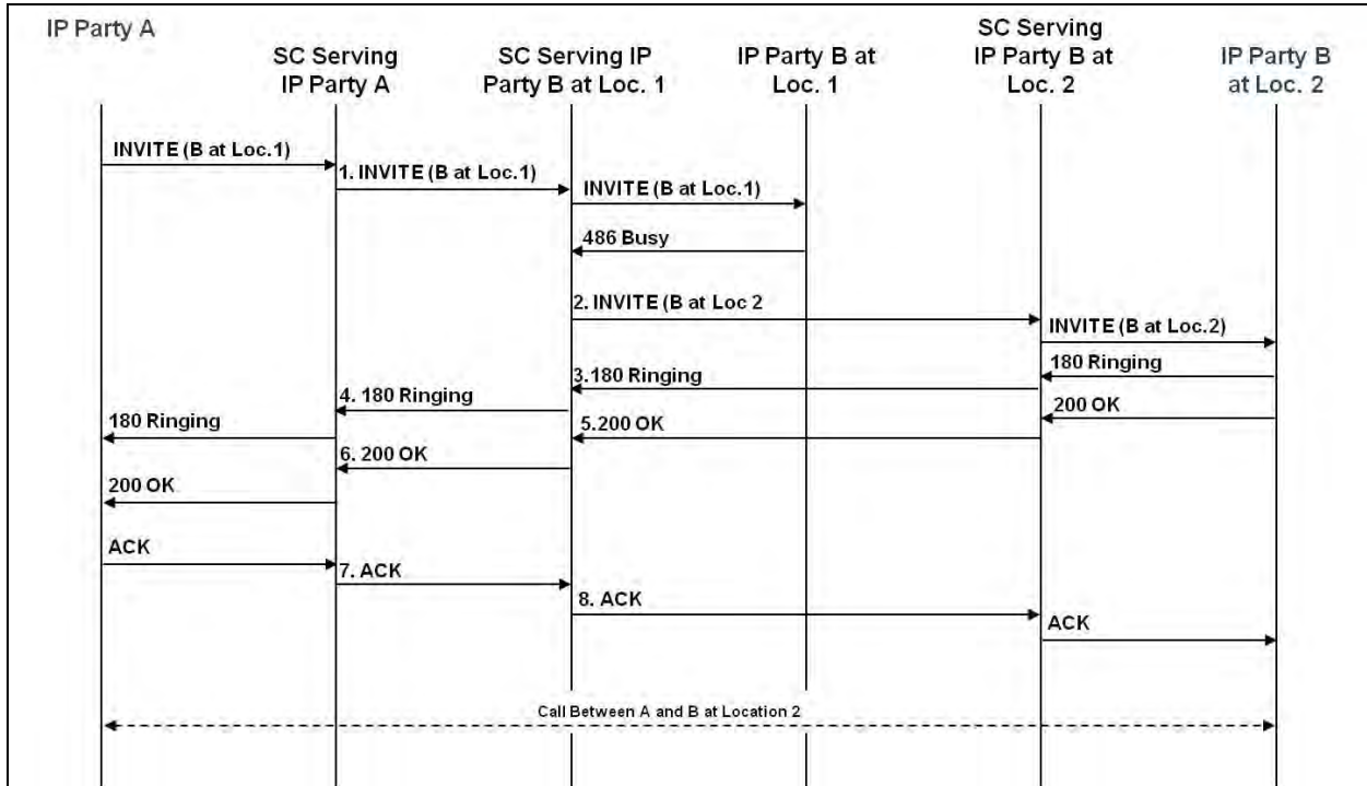
Figure 9.5-9. IP-to-IP Call Forwarding Busy
