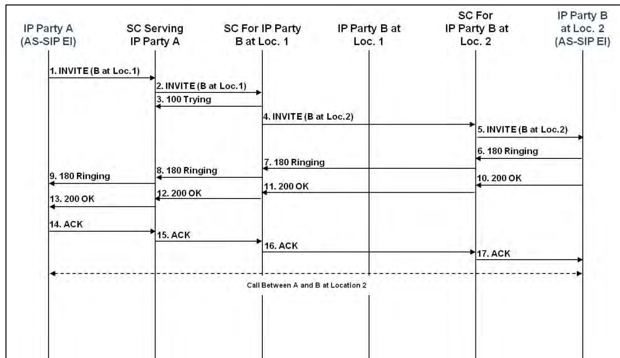
Figure 9.5-4. IP-to-IP Call Forward (Unconditional) (AS-SIP EI)
