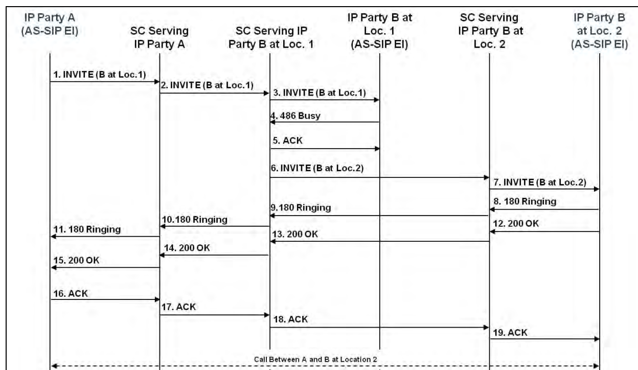
Figure 9.5-12. IP-to-IP Call Forwarding Busy (AS-SIP EI)
