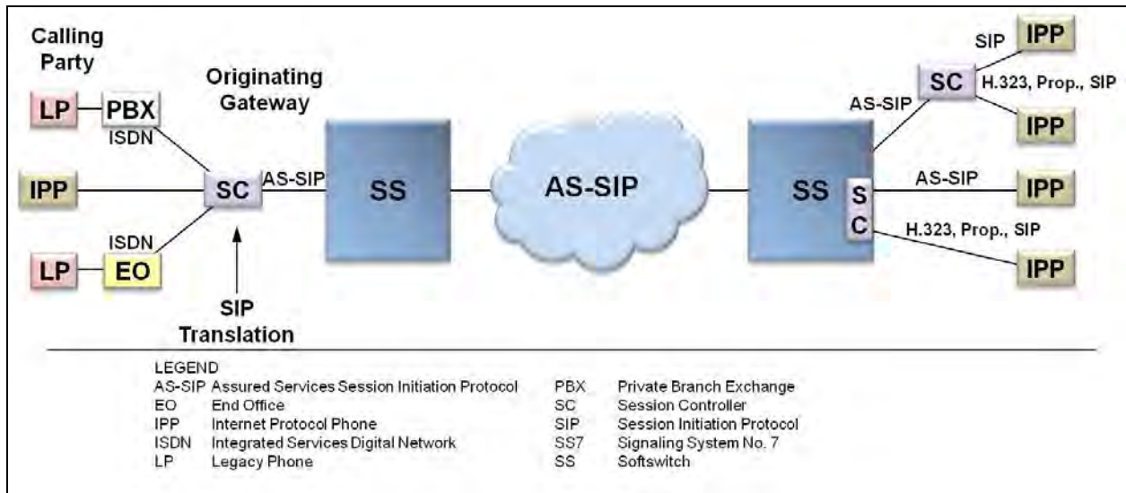
Figure 12.1-6. TDM-to-IP Call Translated at Originating Enclave
