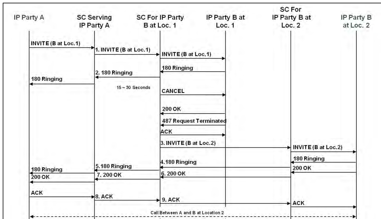
Figure 9.5-5. IP-to-IP Call Forwarding on No Answer
