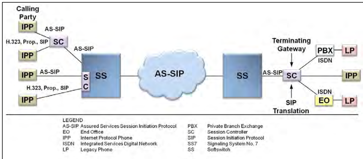
Figure 12.1-8. IP-to-TDM Call Translated at Destination Enclave
