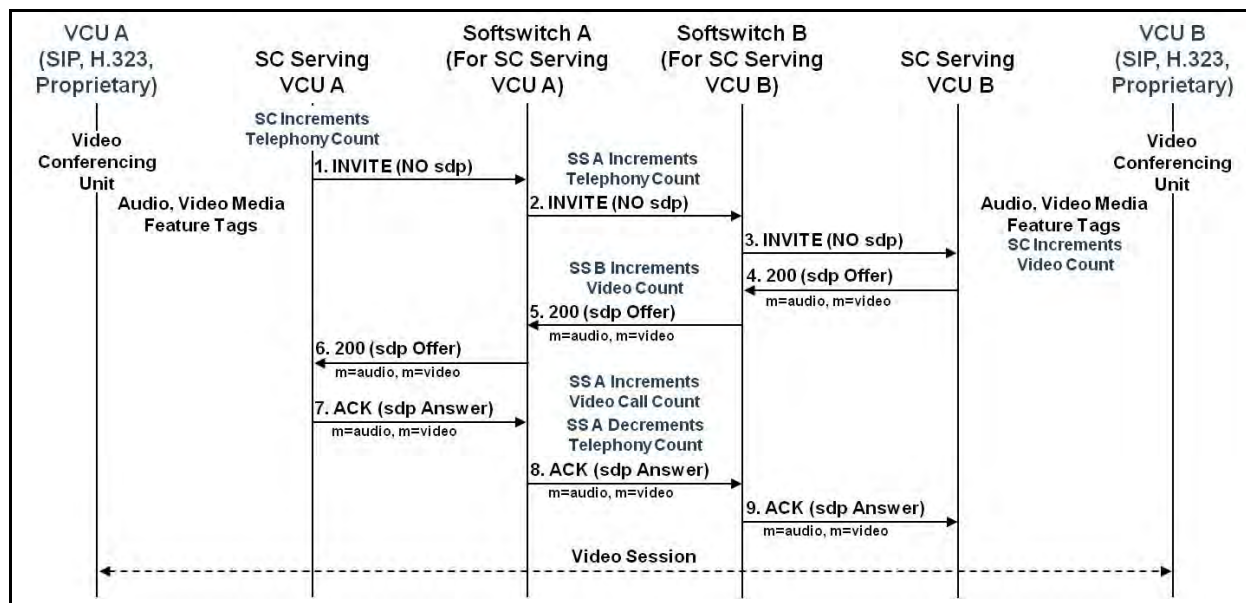
Figure 8.4-5. VCU Empty INVITE (Media Feature Tags Used by Originating SC and Terminating SC)
