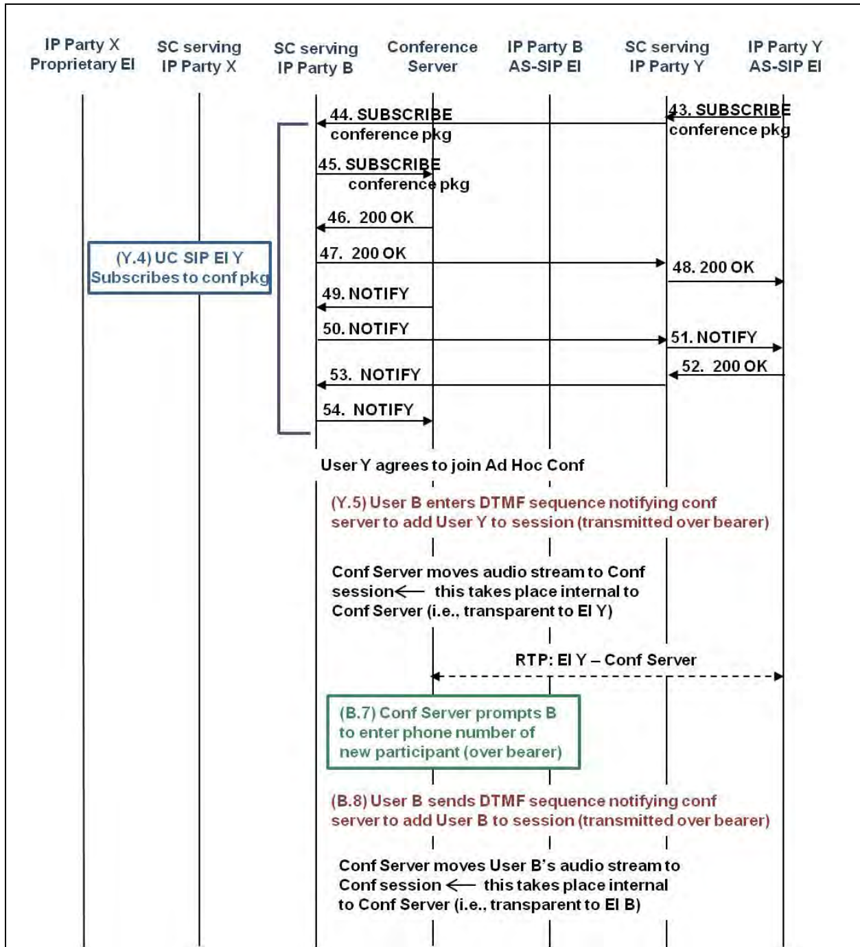
Figure 10.2-12. Ad Hoc Conference – AS-SIP Conference Server, Conference Initiator at AS-SIP EI (Steps 43–54)
