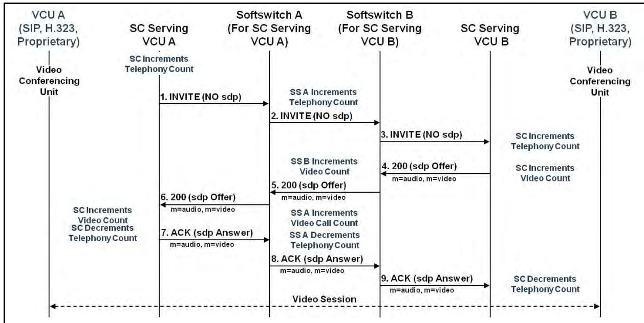
Figure 8.4-3. VCU Empty INVITE (Media Feature Tags NOT Used)
