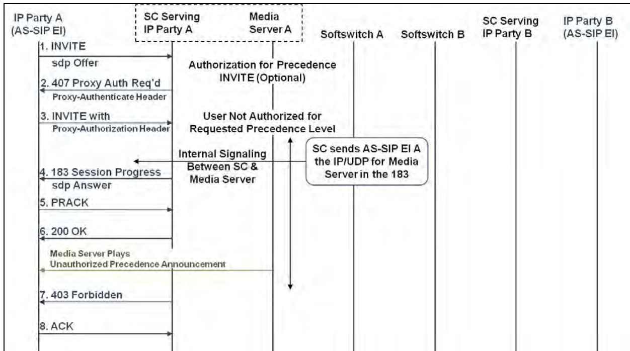
Figure 6.1-1. SC/Media Server Plays UPA to AS-SIP EI (with P&P)
