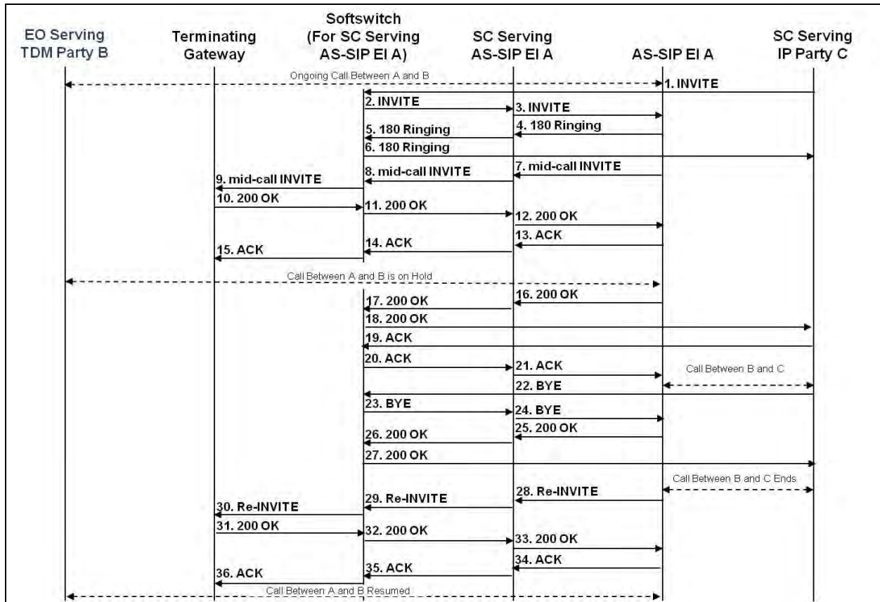
Figure 16.4-8. AS-SIP-TDM Call Waiting (Performed at AS-SIP EI A) (AS-SIP Signaling to AS-SIP EI A Is Depicted for Illustrative Purposes)
