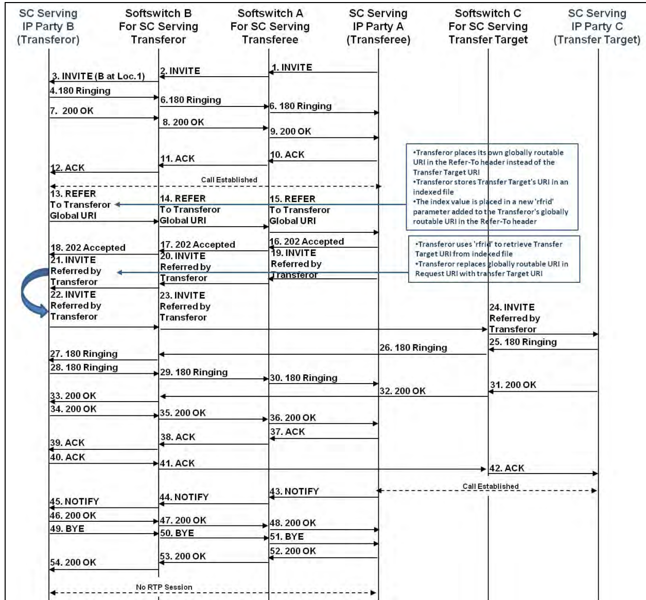
Figure 9.6-1. Unattended Call Transfer for IP EIs (REFER Method)
