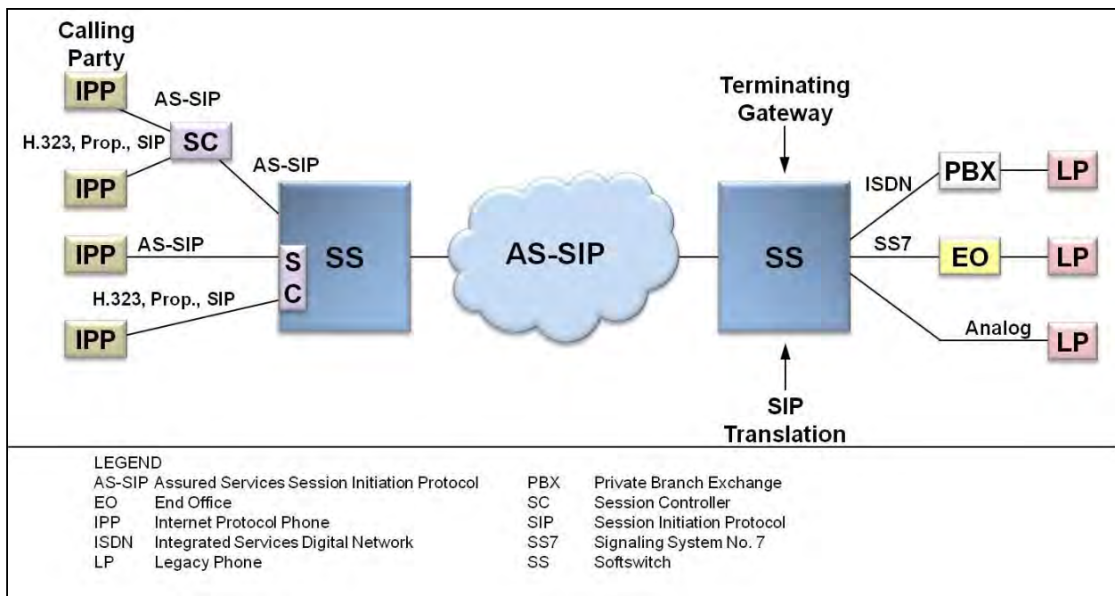
Figure 12.1-7. IP-to-TDM Call Over an IP Backbone
