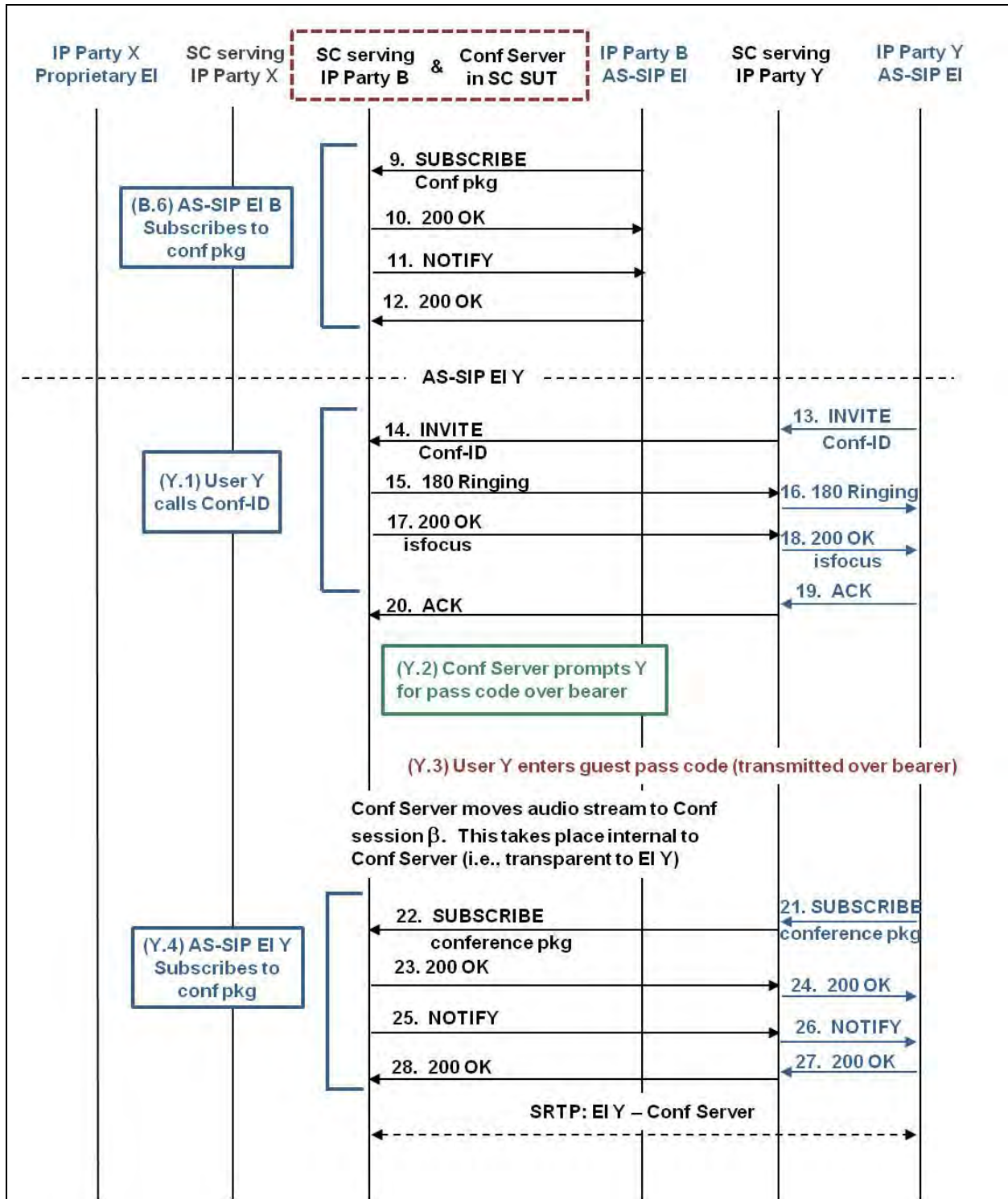
Figure 10.3-3. Scheduled Videoconference – Conference Server Within SC SUT (Steps 9–28)
