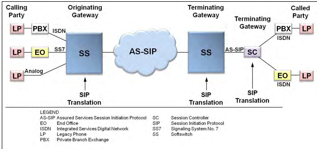
Figure 12.1-3. TDM-to-TDM Bridging From Softswitch-to-SC
