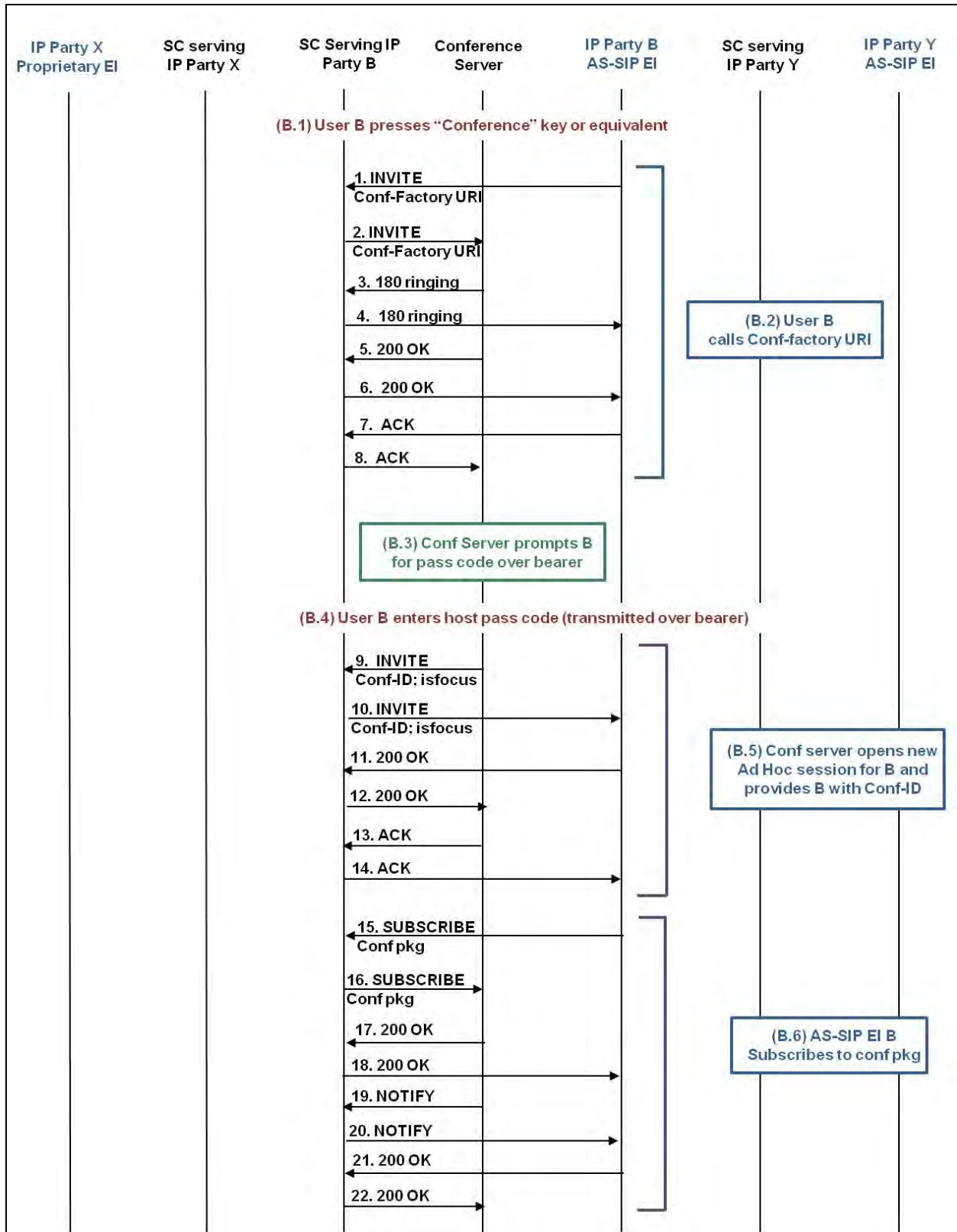
Figure 10.2-10. Ad Hoc Conference – AS-SIP Conference Server, Conference Initiator at AS-SIP EI (Steps 1–22)
