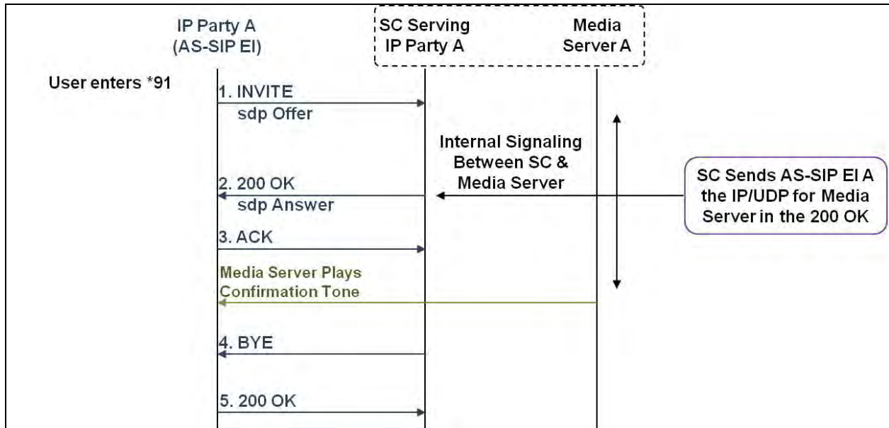
Figure 9.5-11. Call Flow Between AS-SIP EI and SC Using Star Code To Deactivate Call Forward Busy
