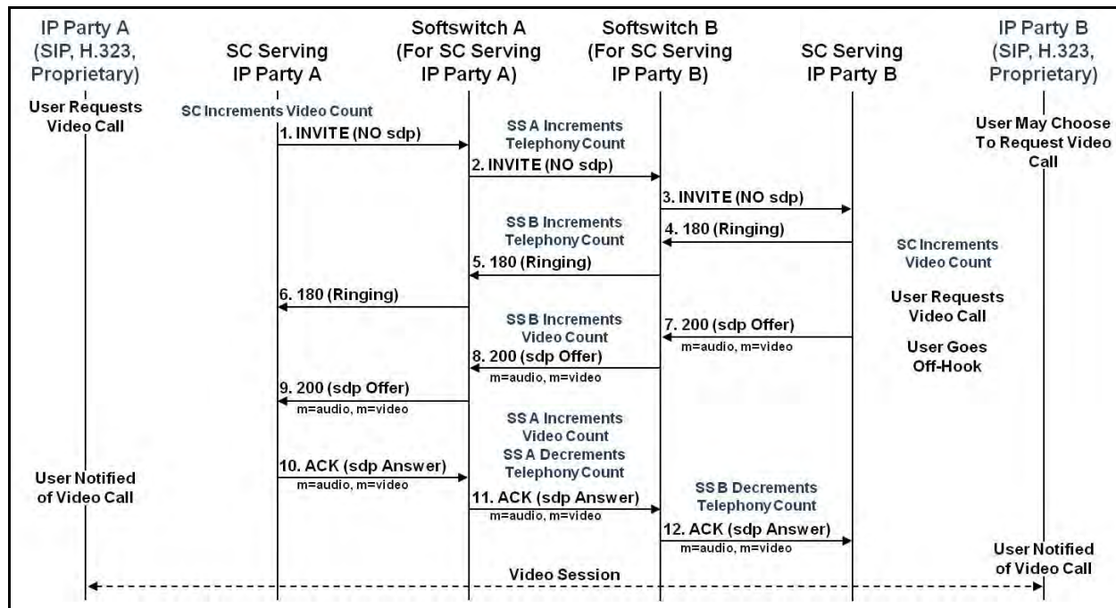
Figure 8.3-9. Empty INVITE – Caller Requests Video; Called Party Offers Video (Media Feature Tags Used by Originating SC and Terminating SC)
