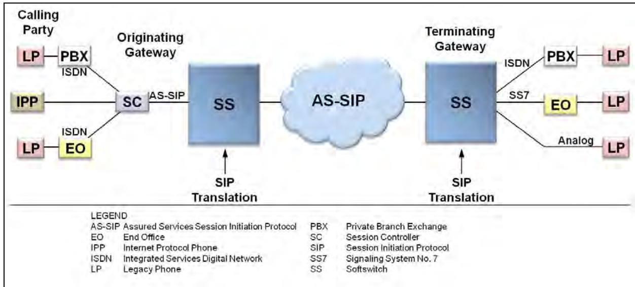
Figure 12.1-4. TDM-to-TDM Bridging From SC-to-Softswitch
