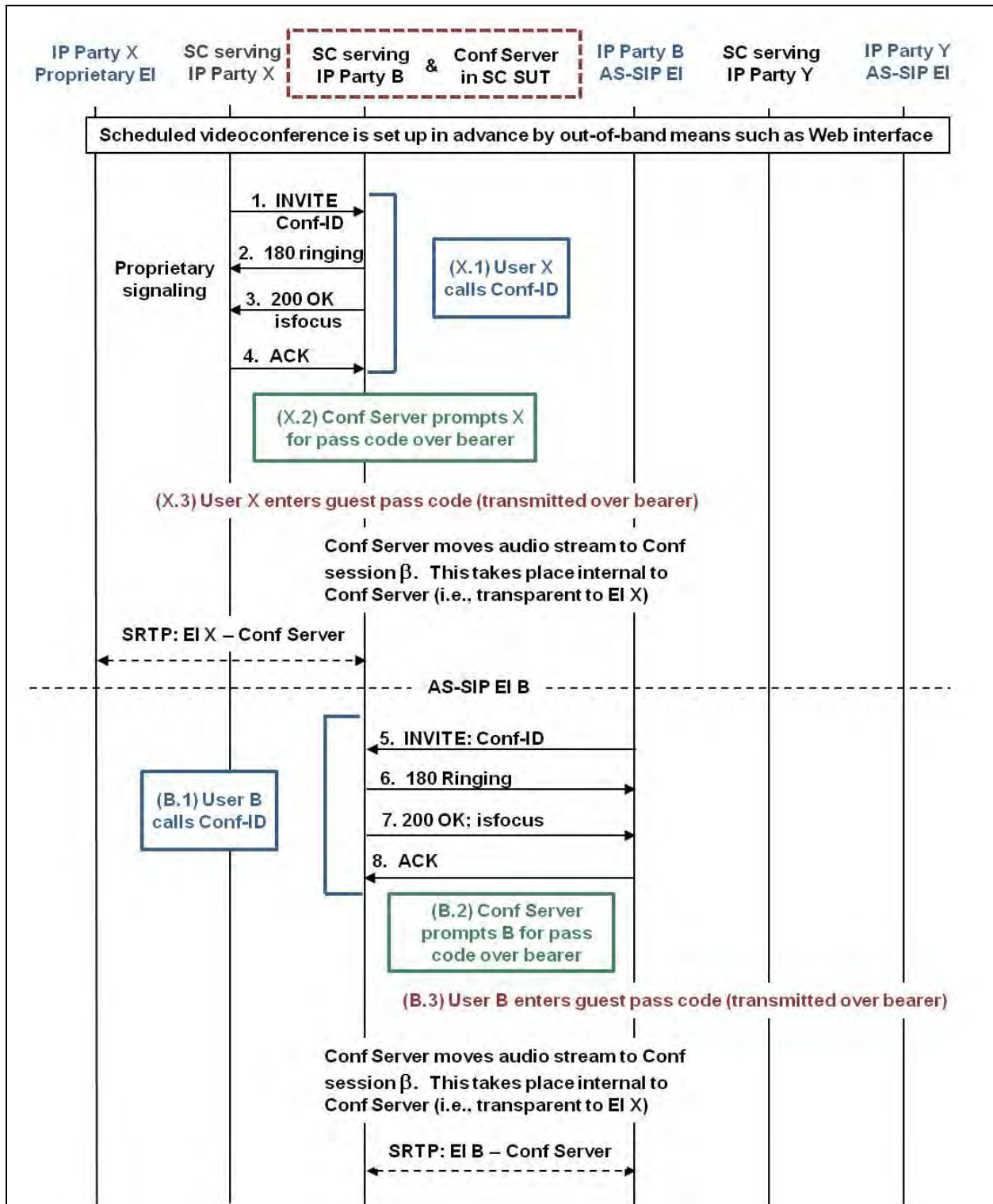
Figure 10.3-2. Scheduled Videoconference – Conference Server Within SC SUT (Steps 1–8)
