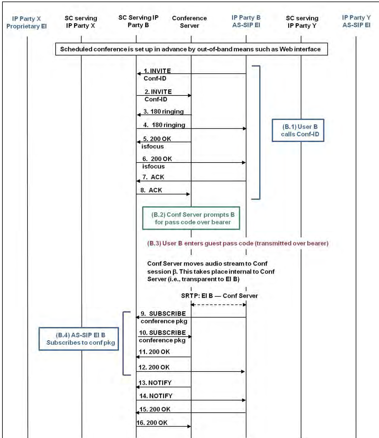
Figure 10.2-28. Scheduled Conference – AS-SIP Conference Server, Host at AS-SIP EI (Steps 1–16)
