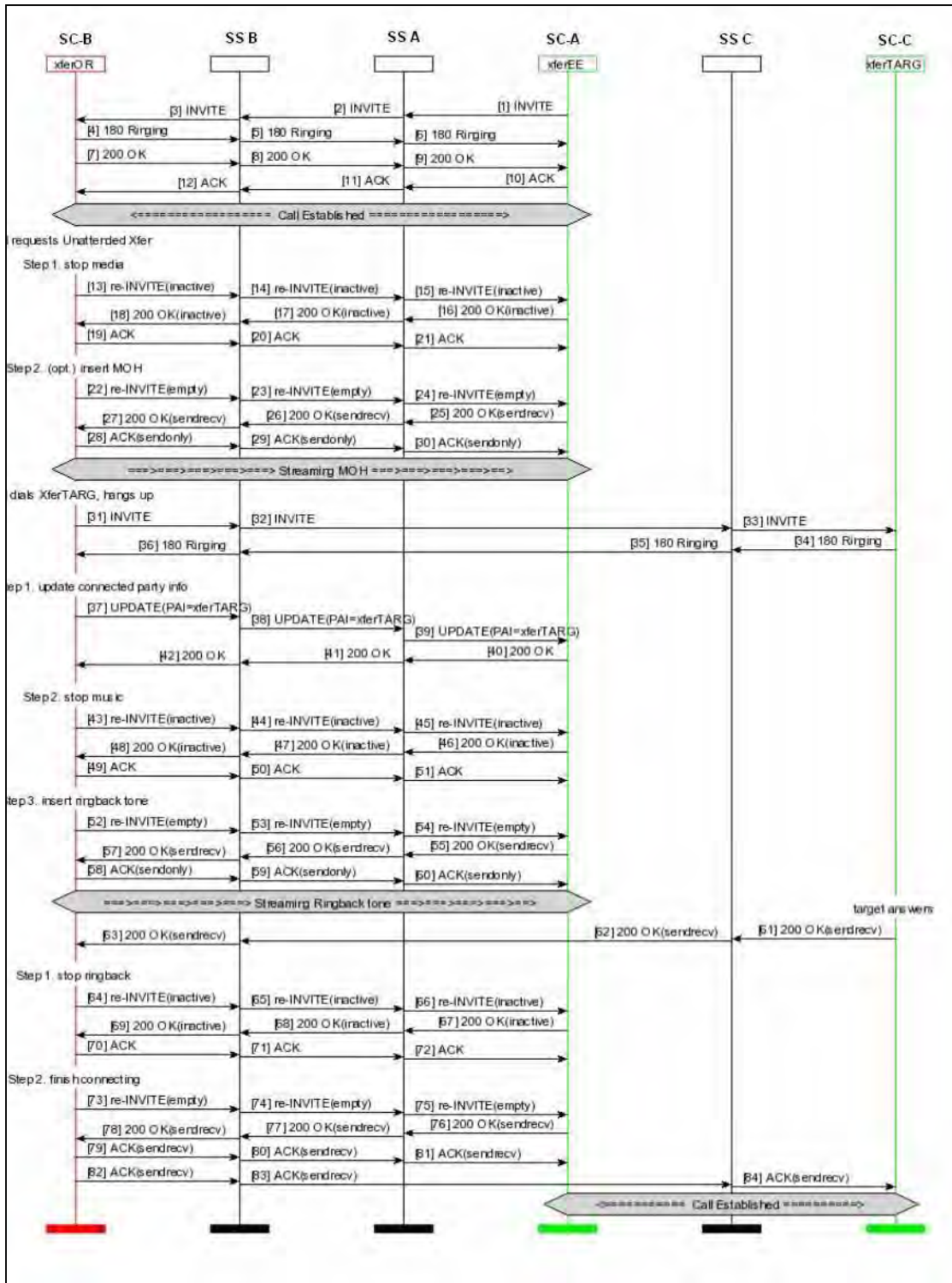
Figure 9.6-2. Unattended Call Transfer for IP EIs (INVITE and re-INVITE Method)
