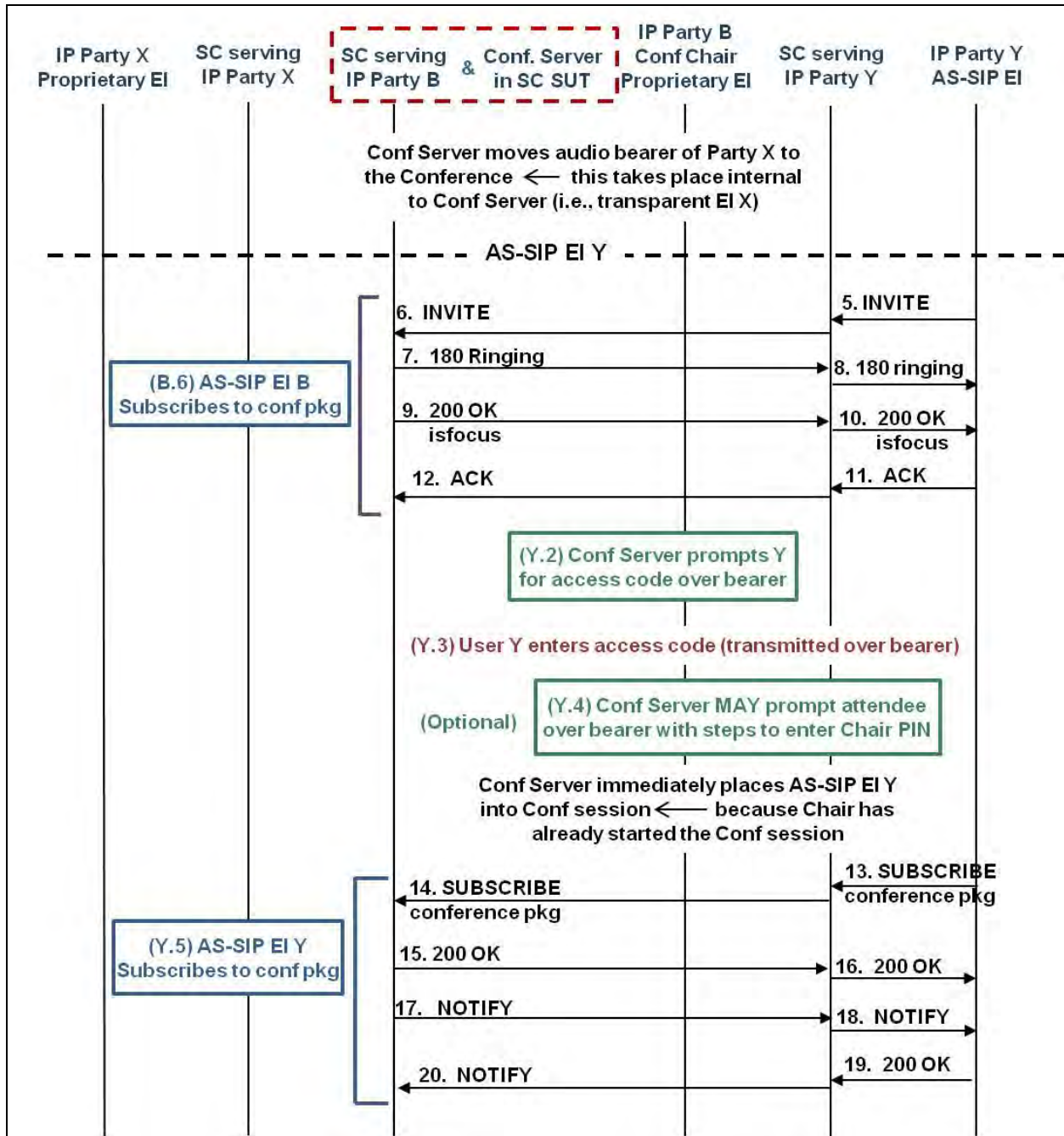
Figure 10.2-14. Reservationless Conference – Conference Server Within SC SUT, Conference Chair at Proprietary EI (Steps 5–20)
