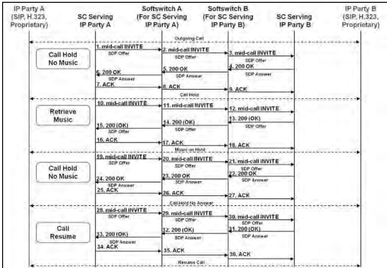
Figure 9.3-5. IP-to-IP Music on Hold (Populated INVITES and Empty INVITES)
