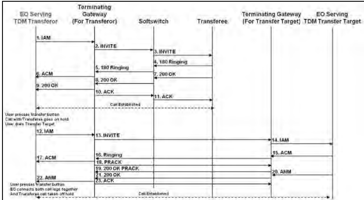
Figure 16.6-2. Attended Call Transfer Transferor – TDM
