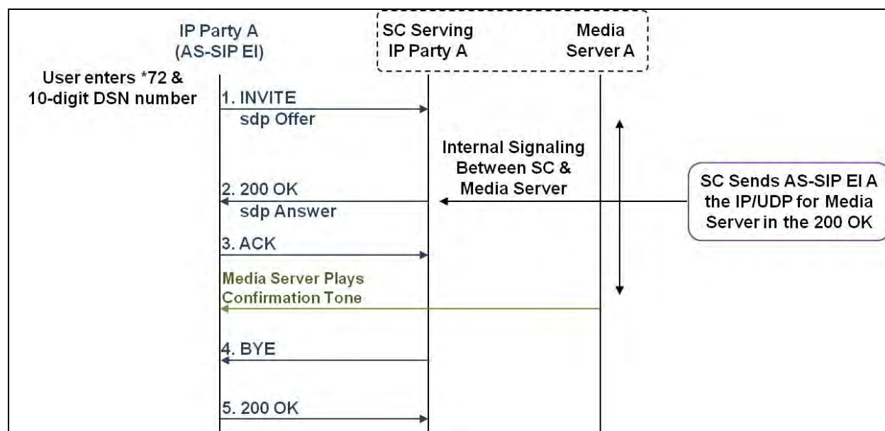
Figure 9.5-2. Call Flow Between AS-SIP EI and SC Using Star Code To Unconditionally Call Forward to a DSN Phone Number
